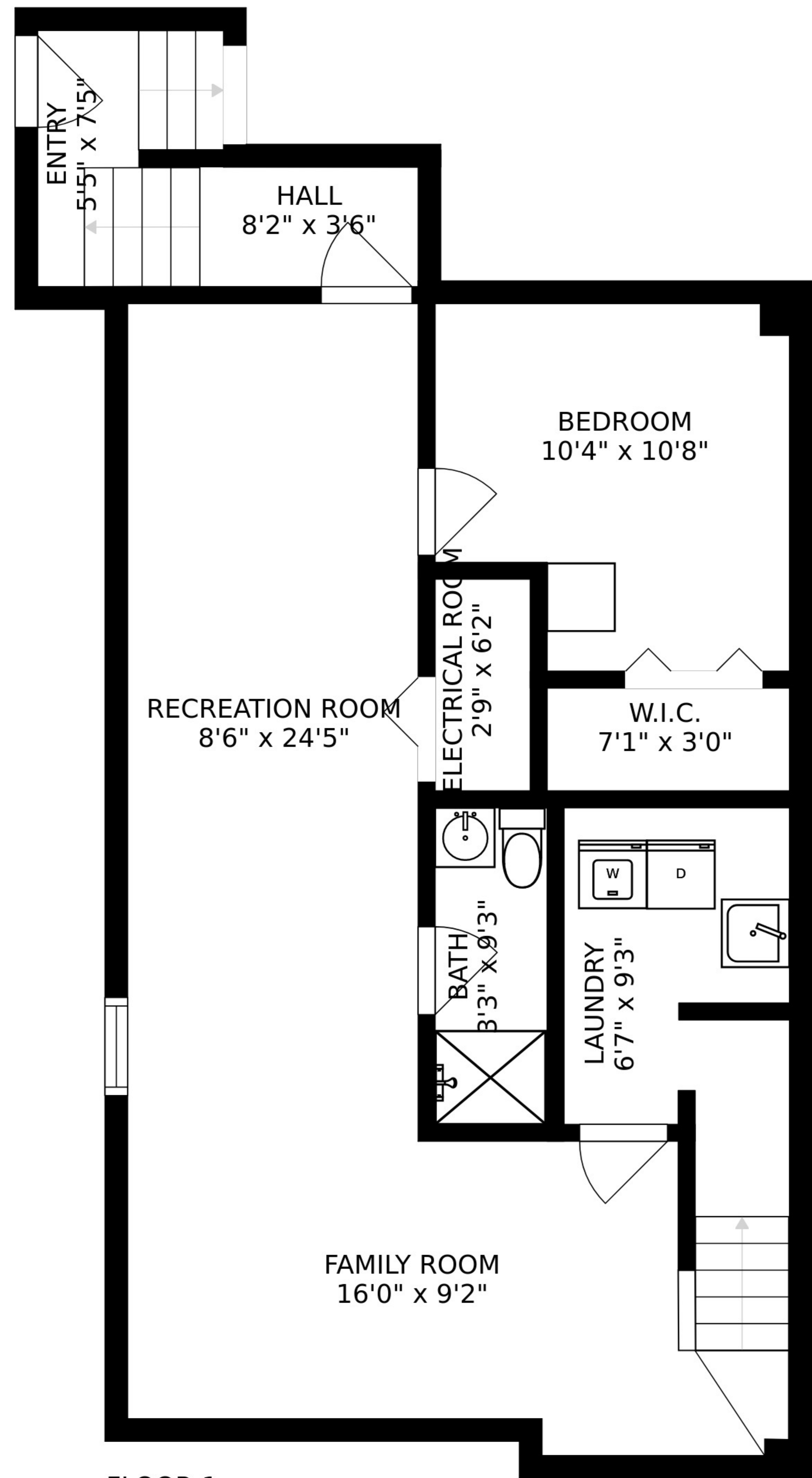
FLOOR 1
