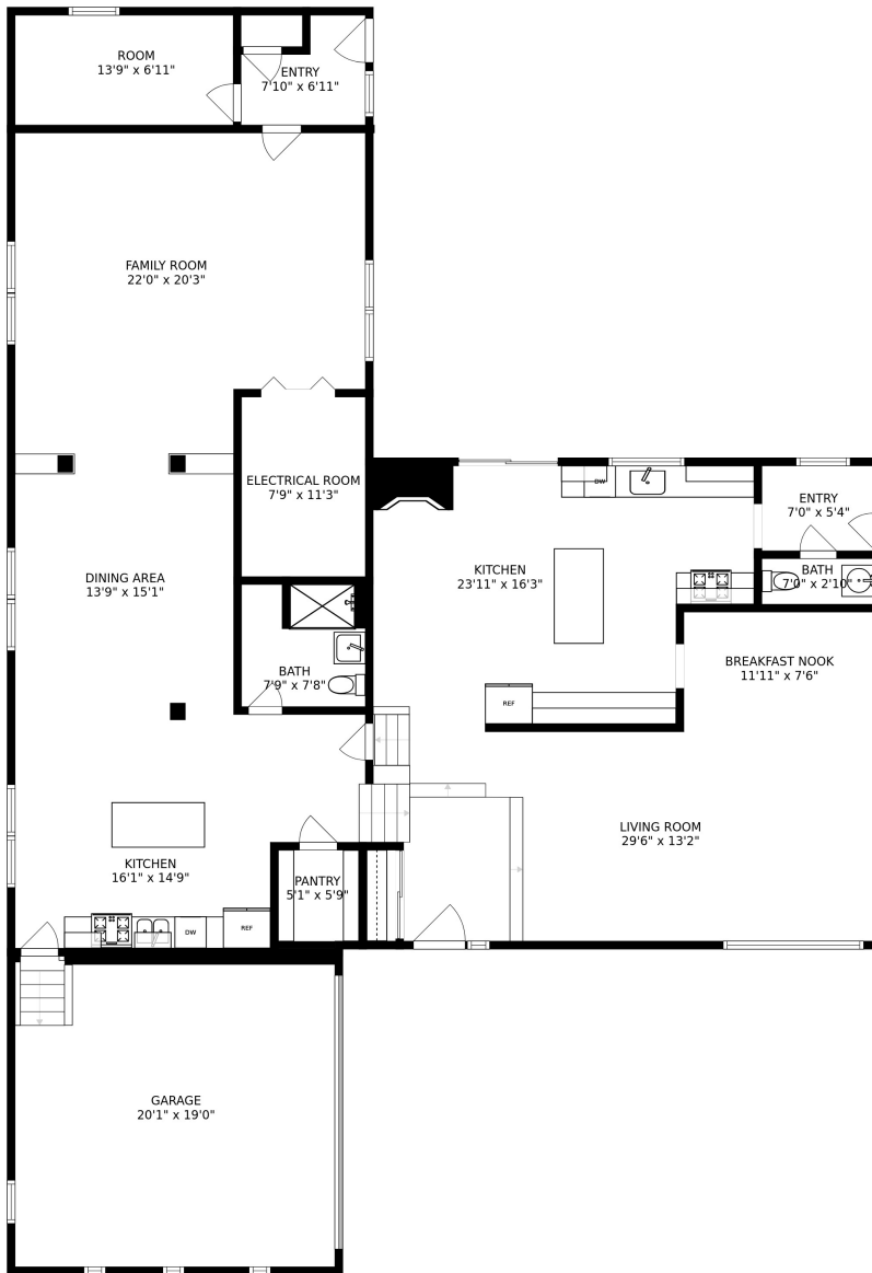
FLOOR 1
