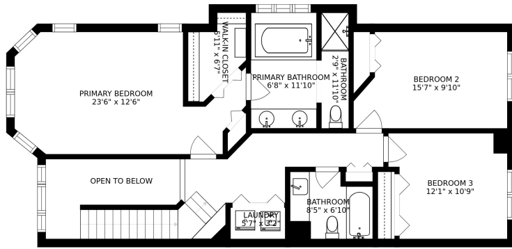
SECOND FLOOR
