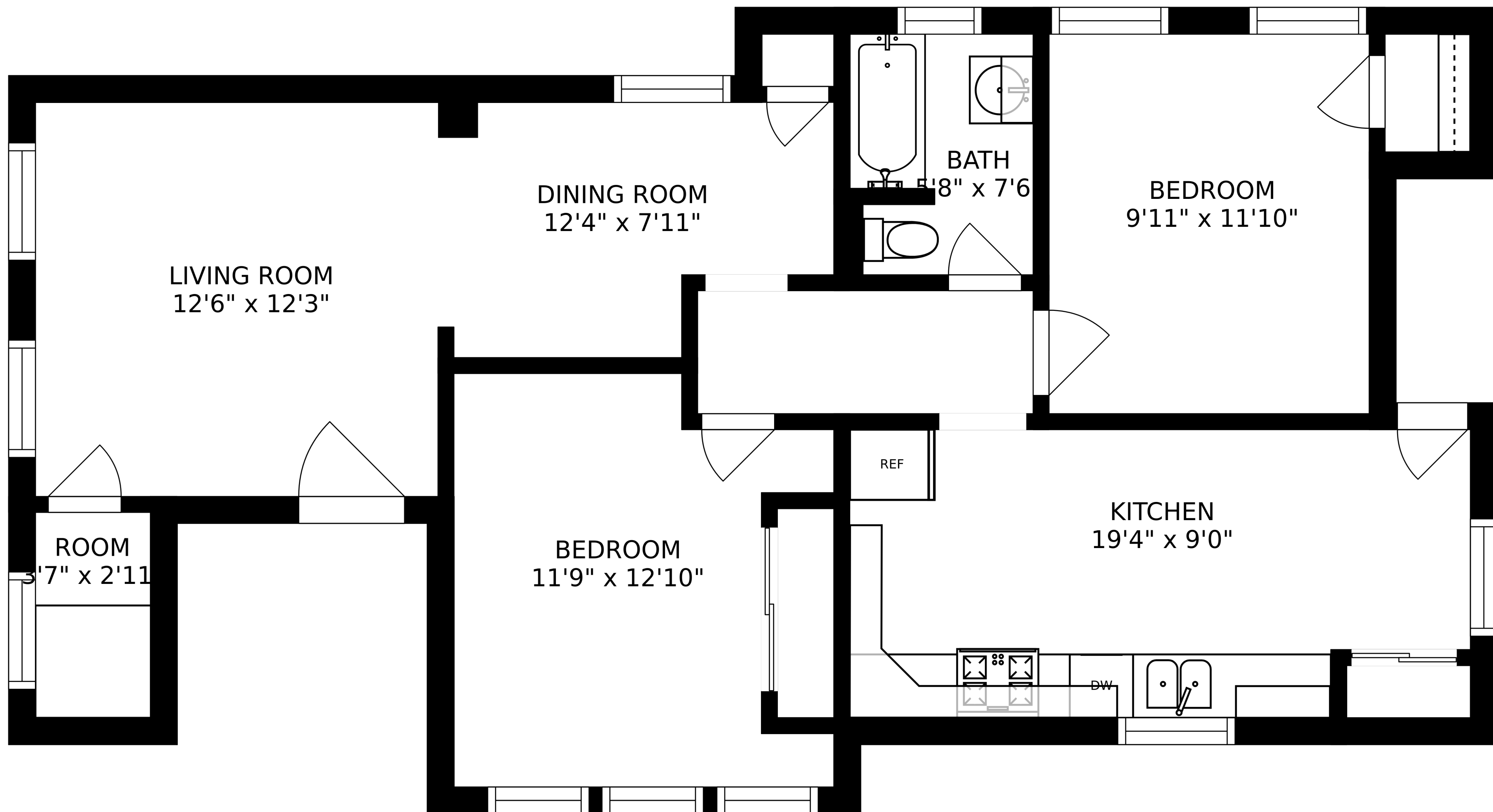
FLOOR 1
