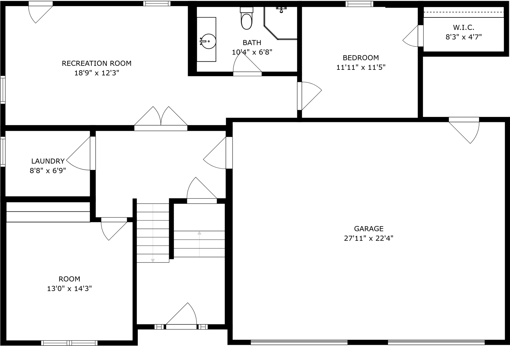
FLOOR 1
