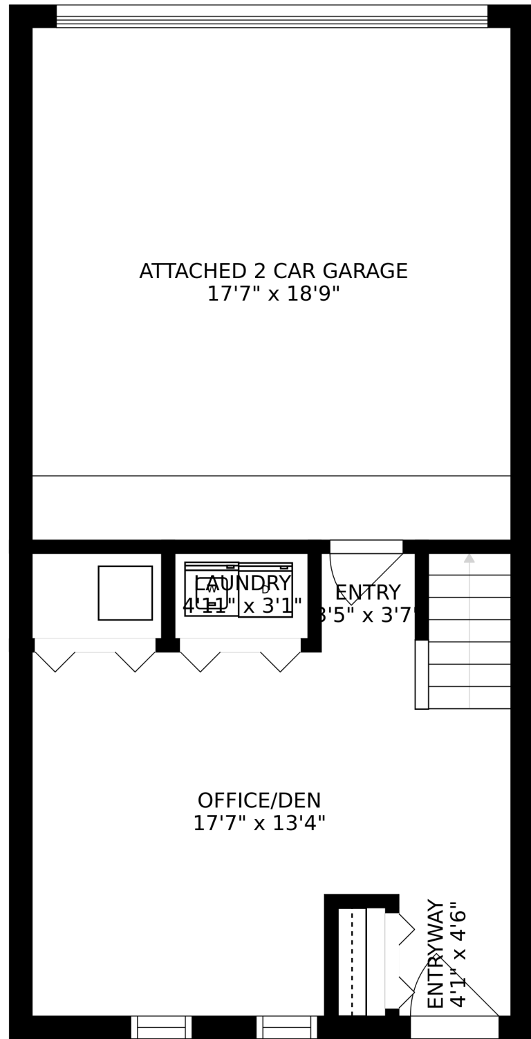
FLOOR 1
