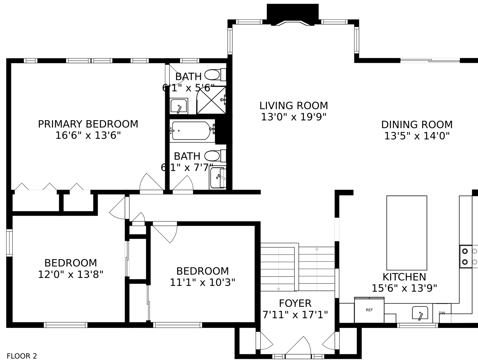
FLOOR 2
