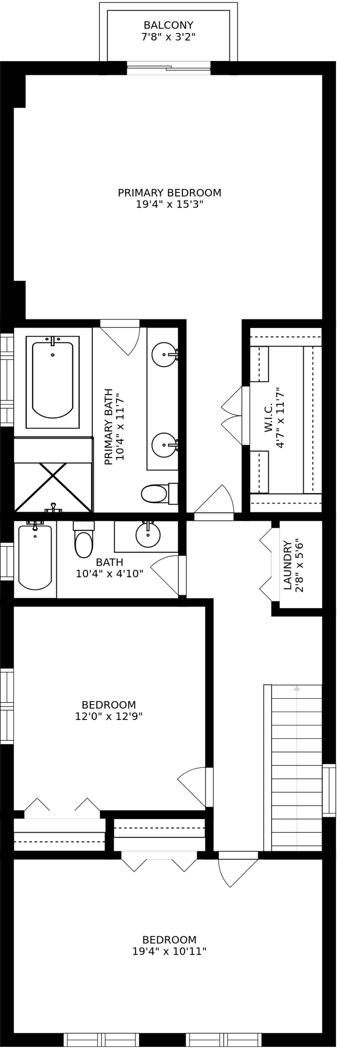
FLOOR 3
