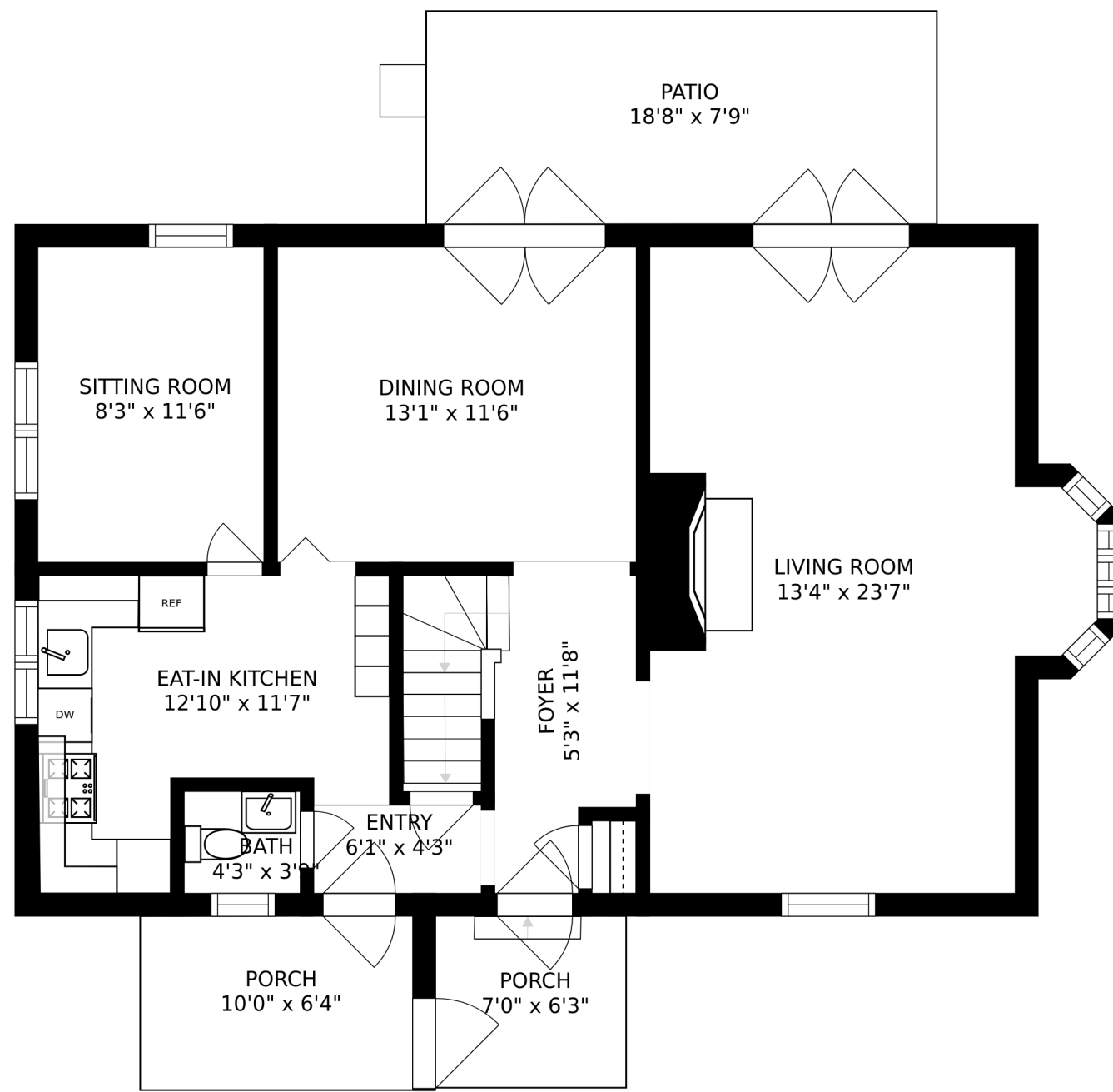
FLOOR 2
