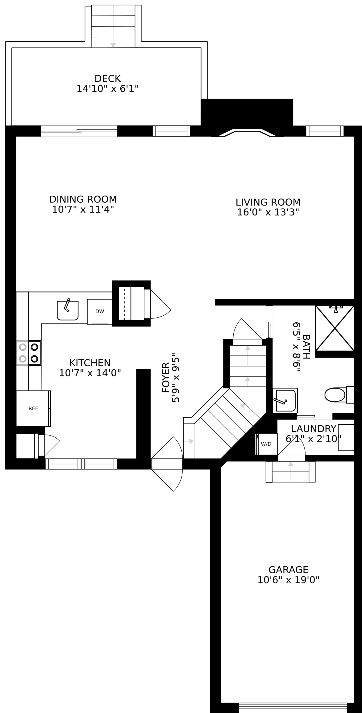
FLOOR 1
