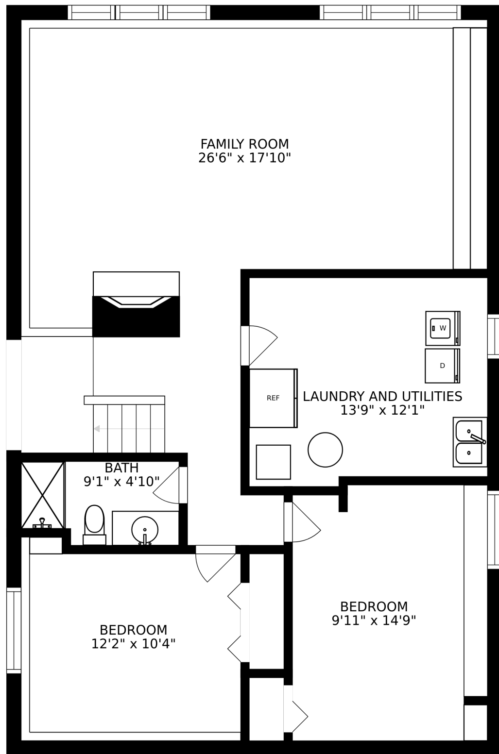
FLOOR 1
