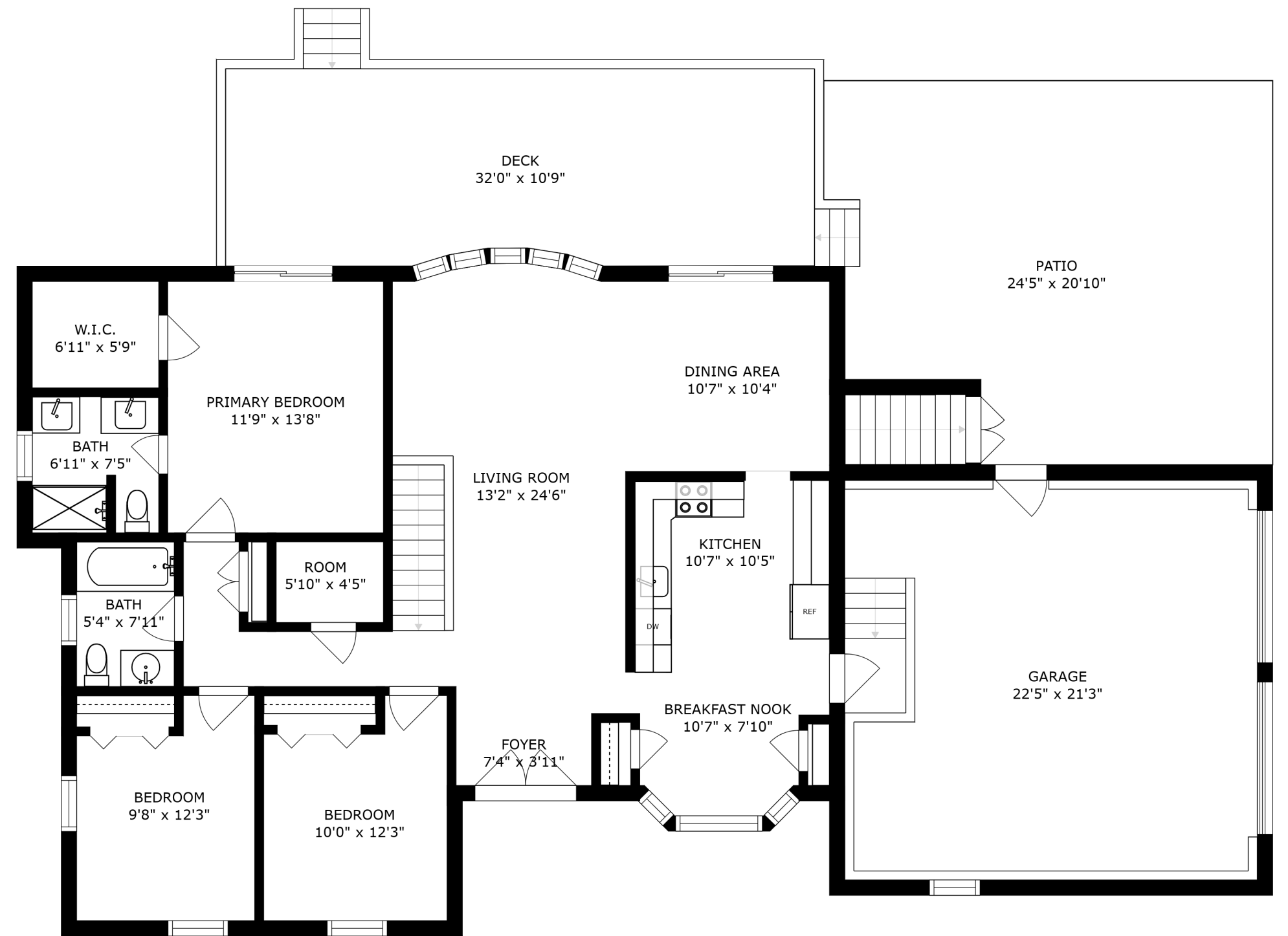
FLOOR 2
