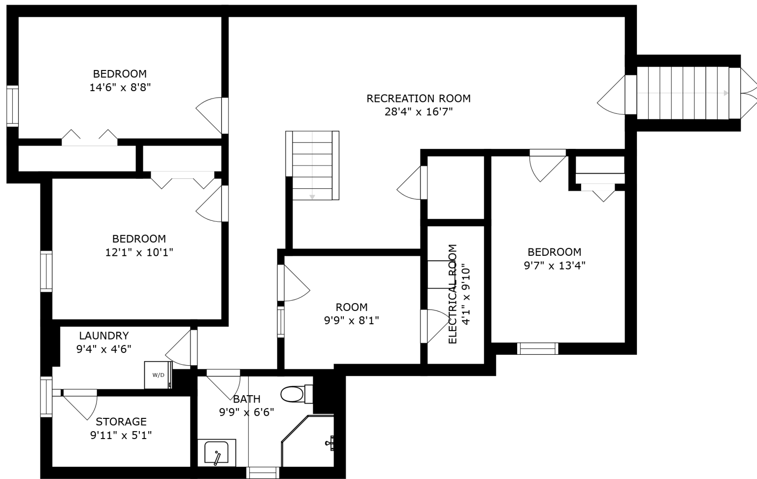
FLOOR 1
