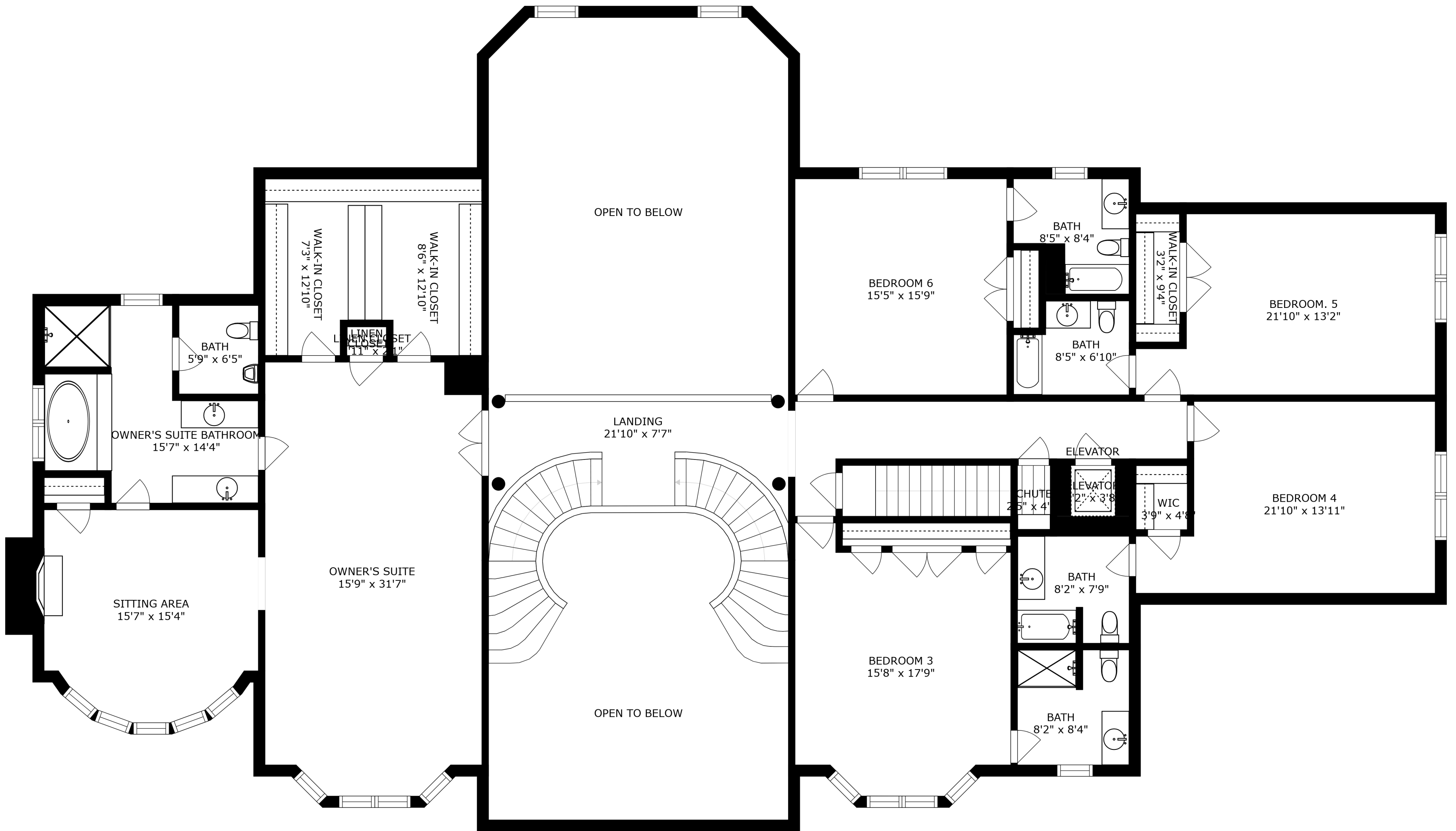
SECOND FLOOR
