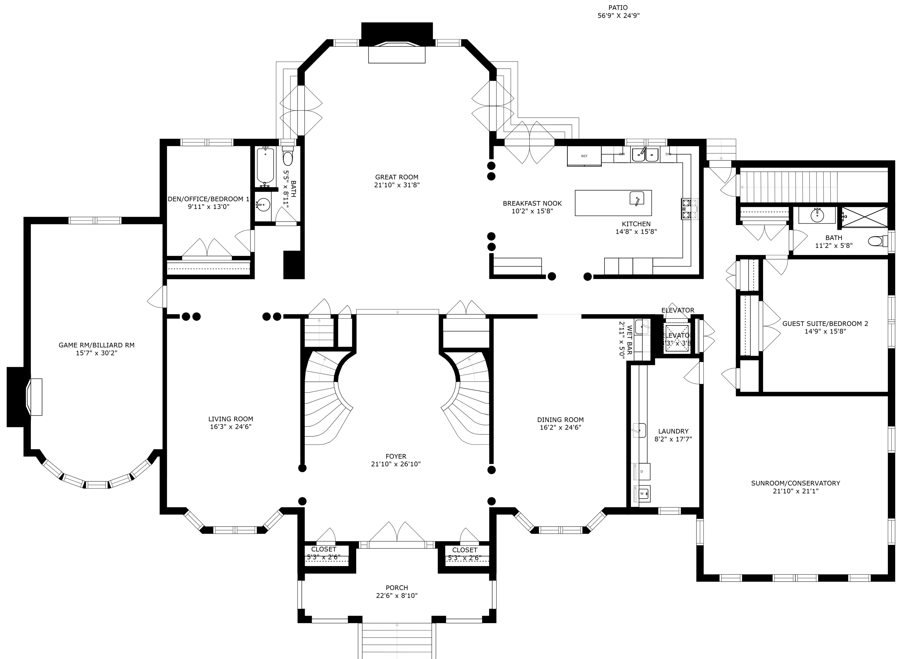
MAIN(FIRST) FLOOR
