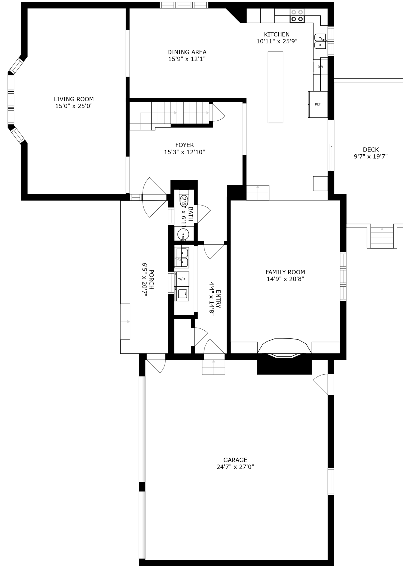
FLOOR 2
