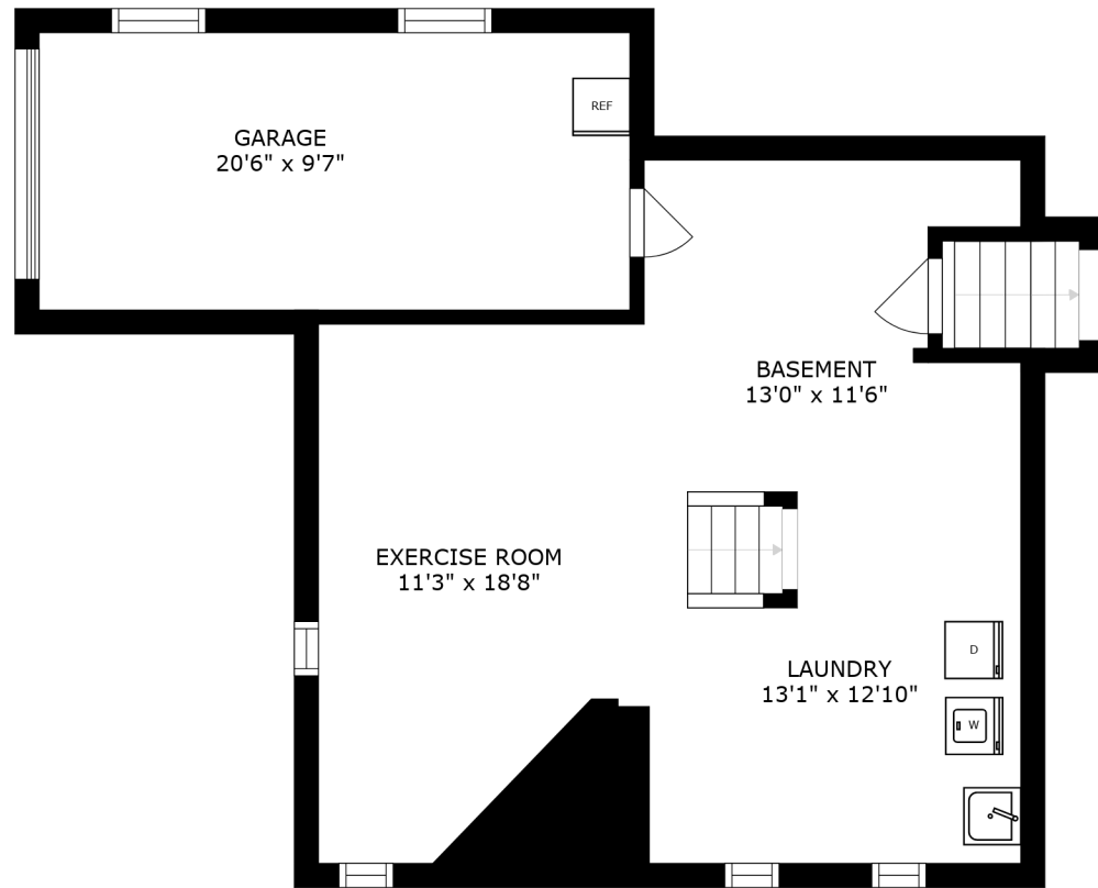
FLOOR 1
