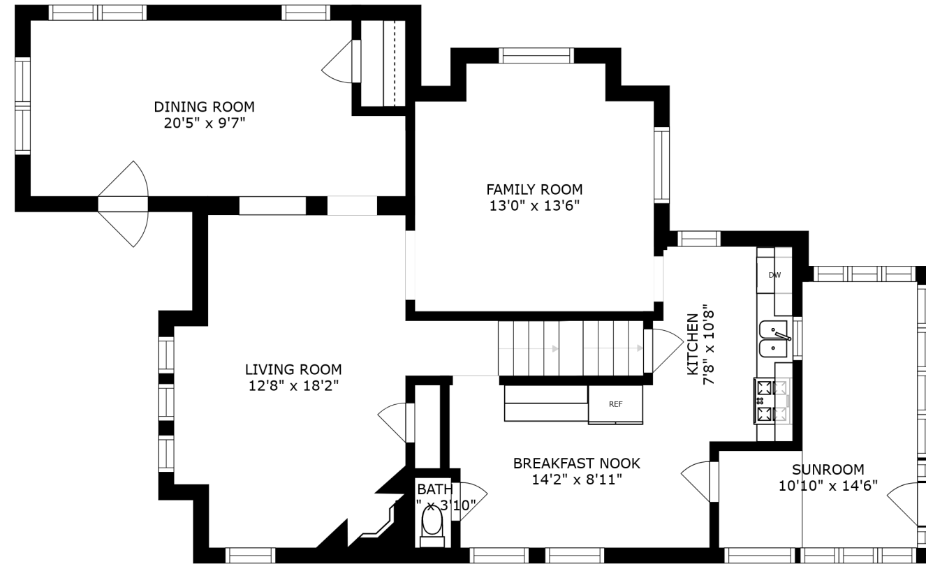
FLOOR 2
