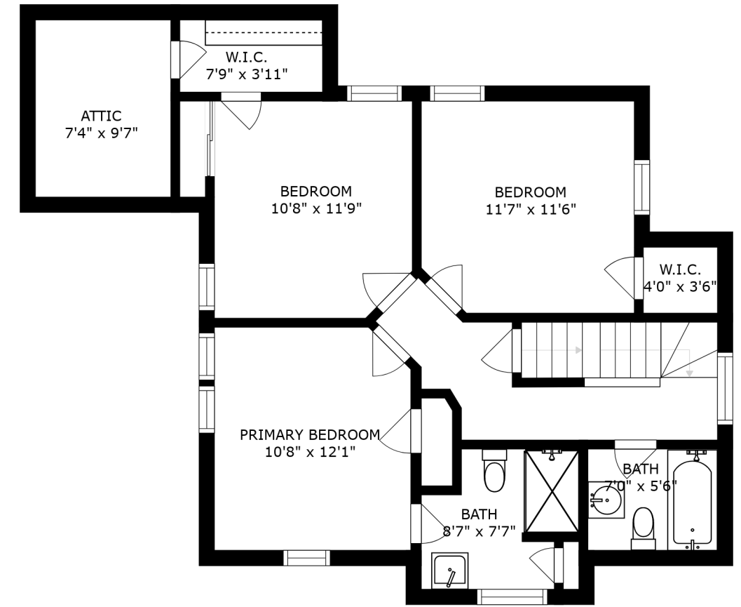
FLOOR 3
