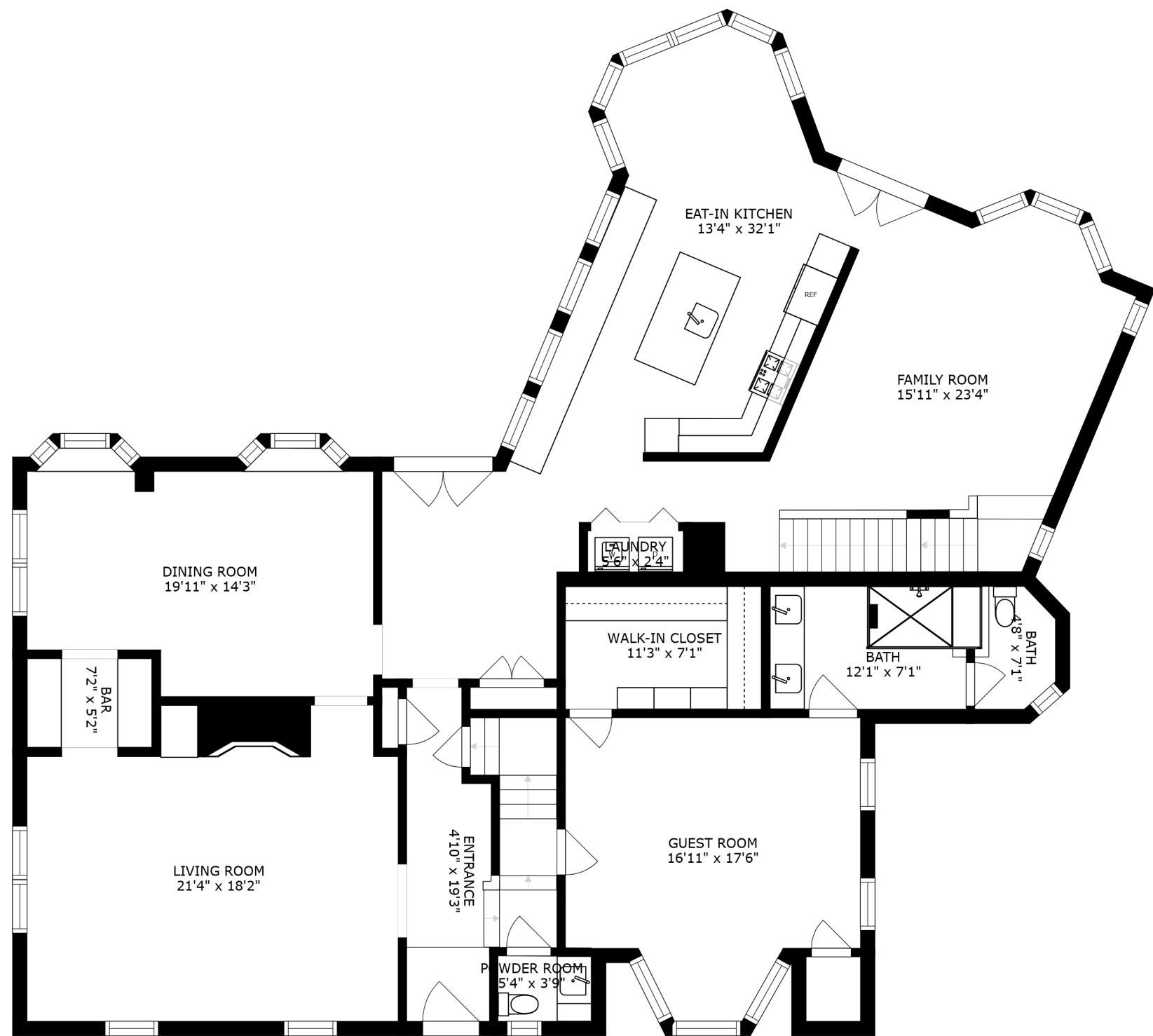
FLOOR 2
