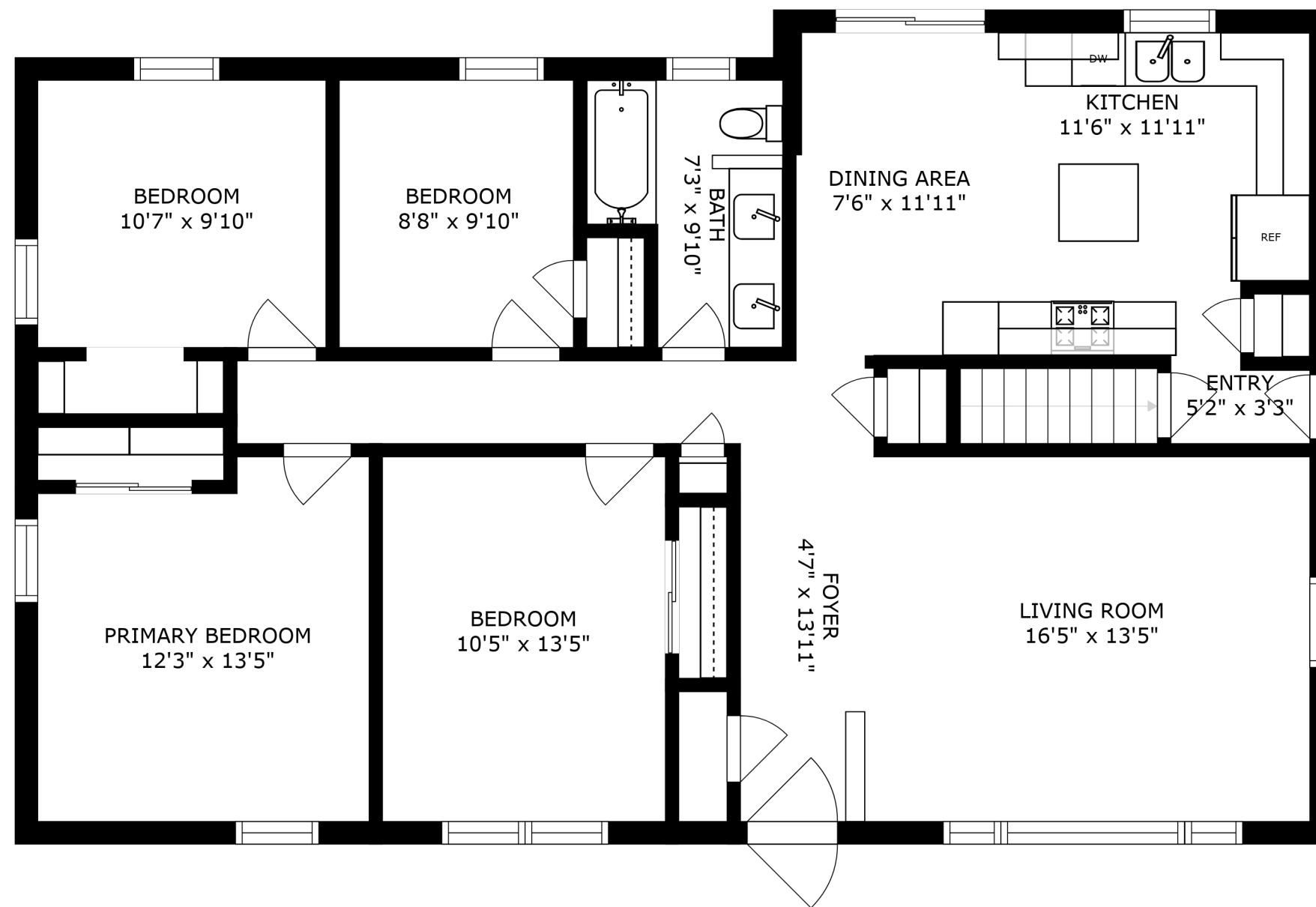
FLOOR 2
