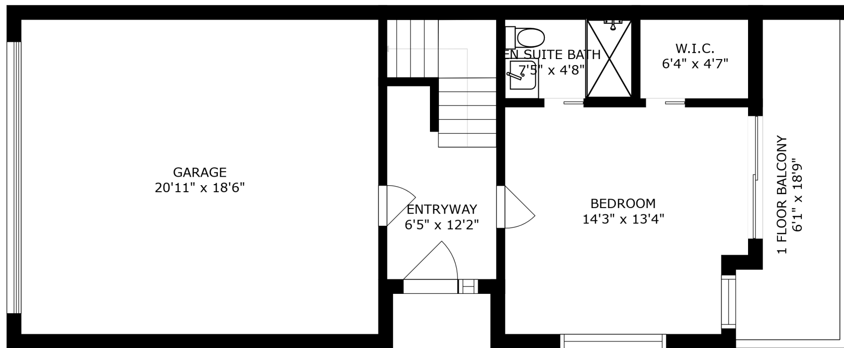
FLOOR 1
