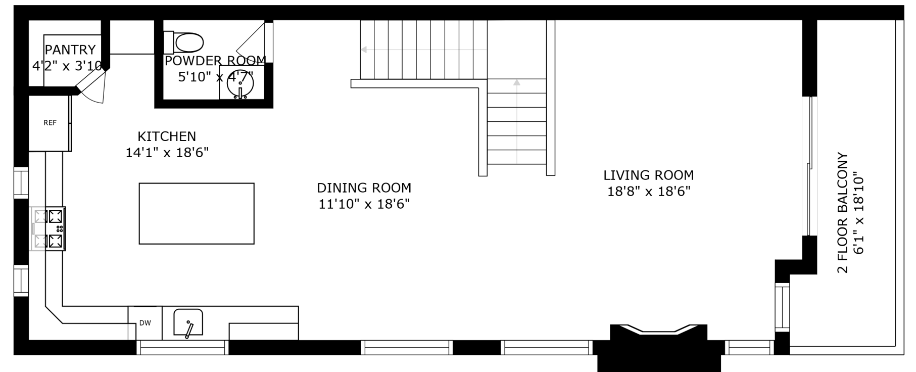
FLOOR 2
