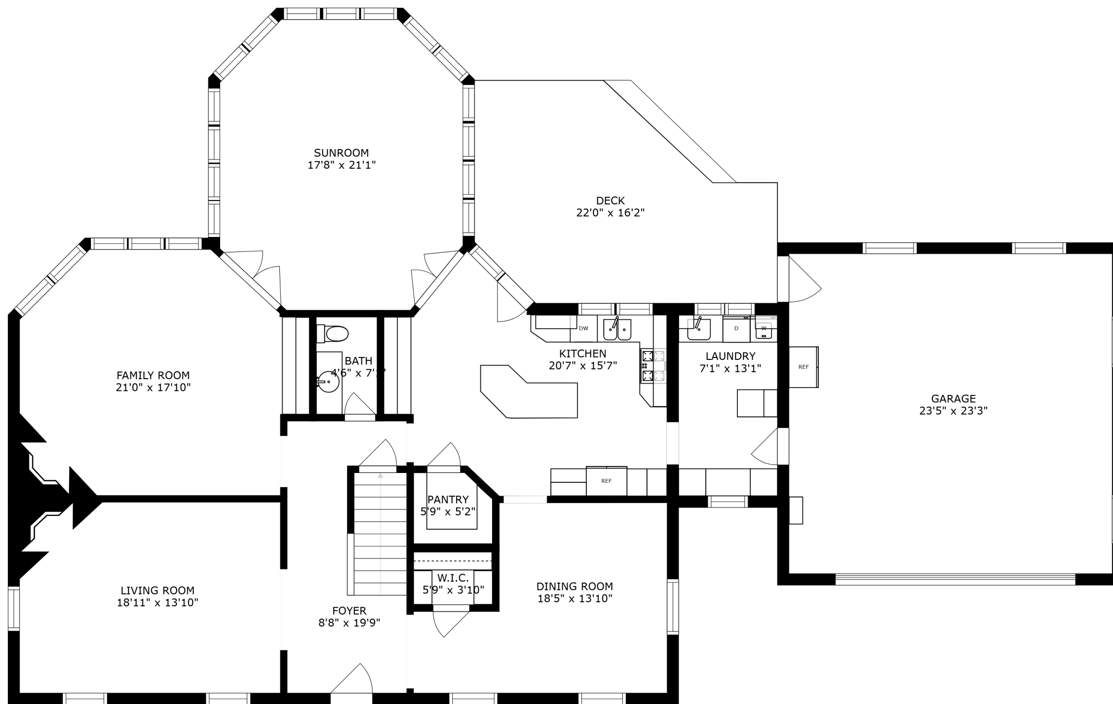
FLOOR 2
