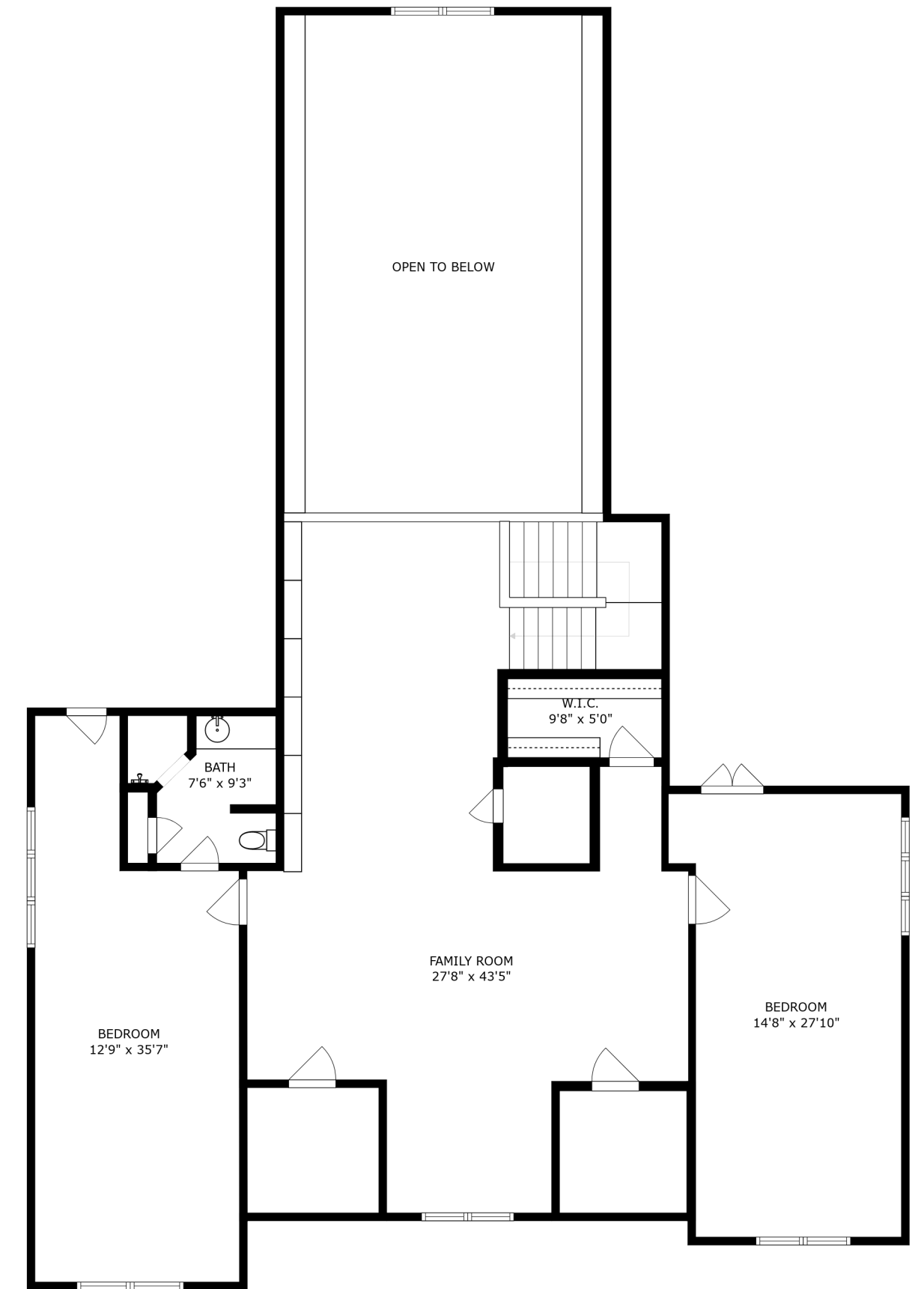
FLOOR 3
