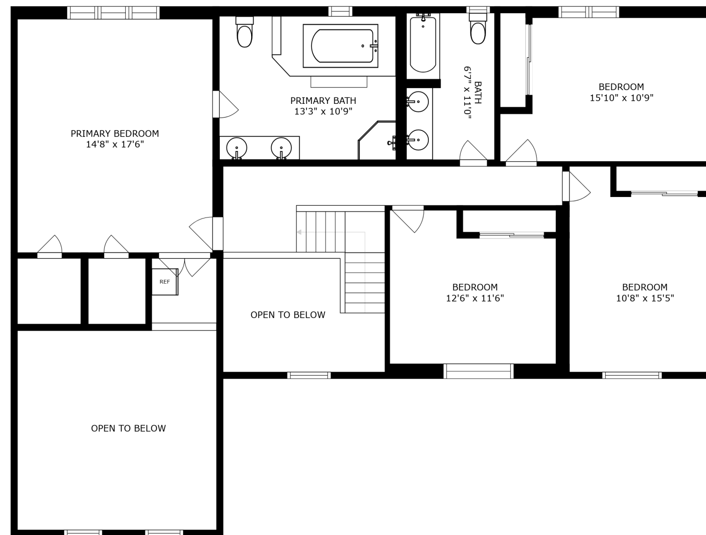
FLOOR 3
