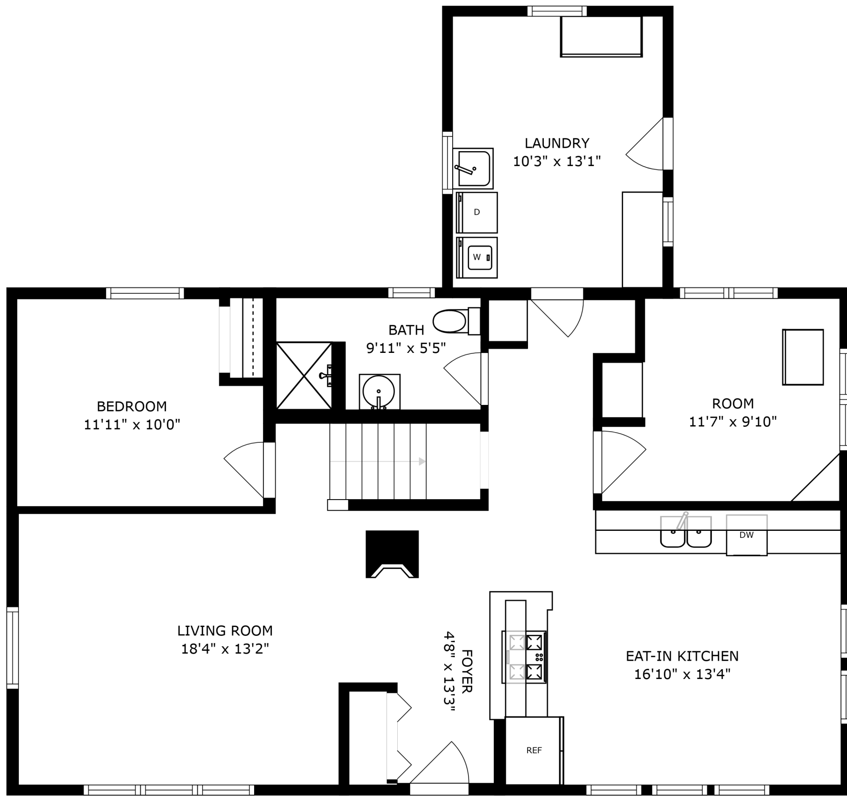
FLOOR 1
