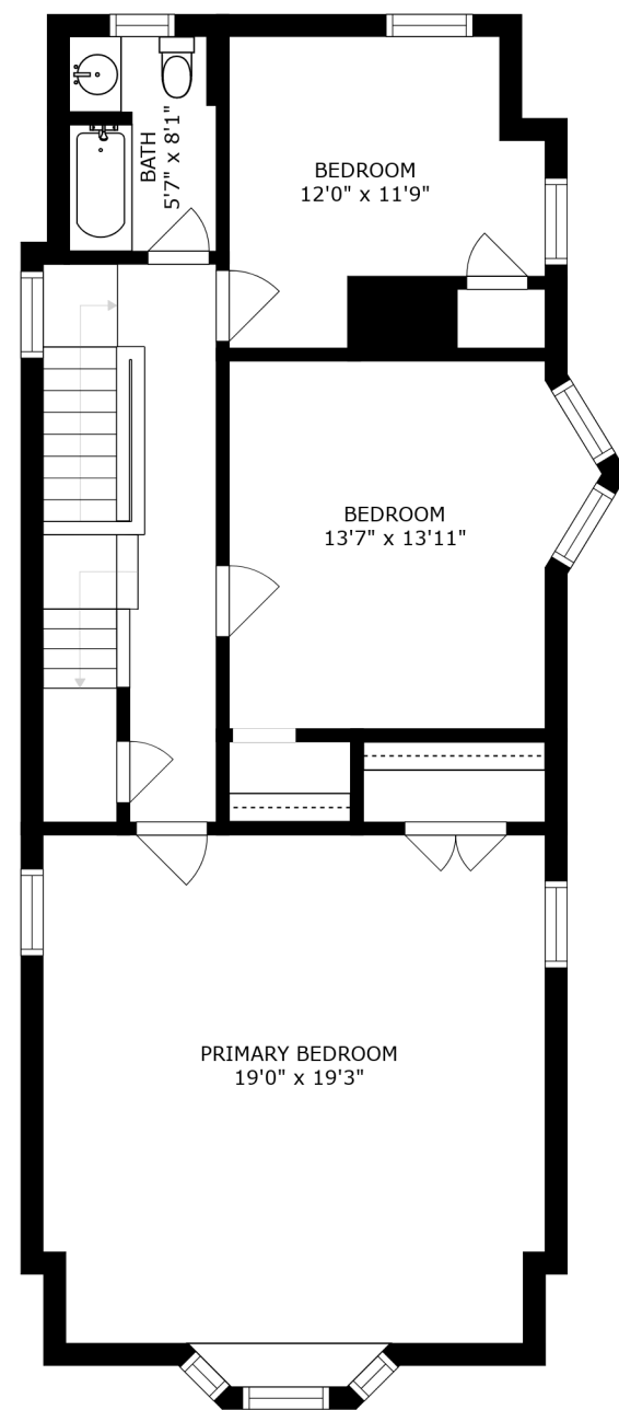
SECOND FLOOR
