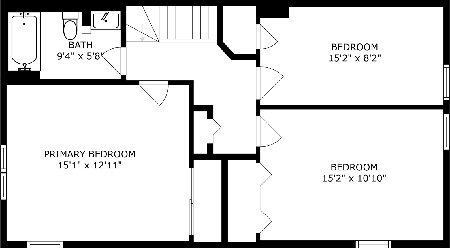
FLOOR 3
