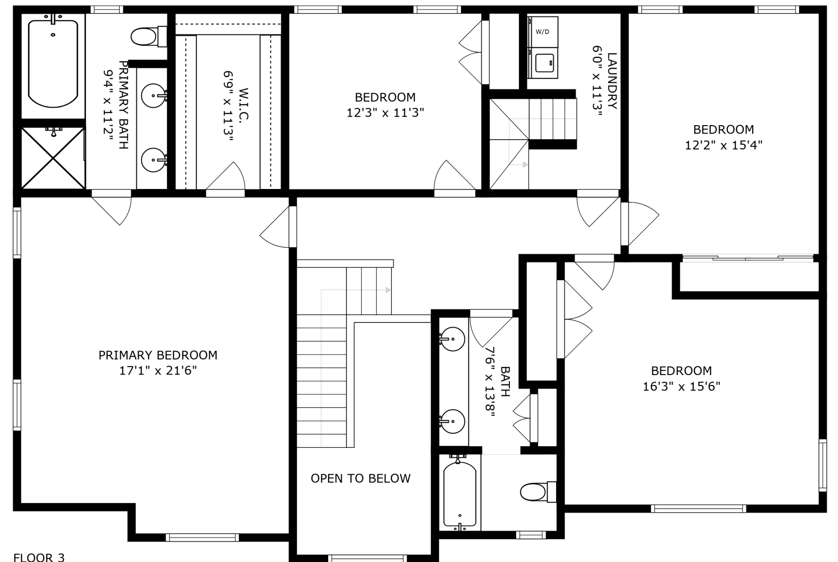
FLOOR 3
