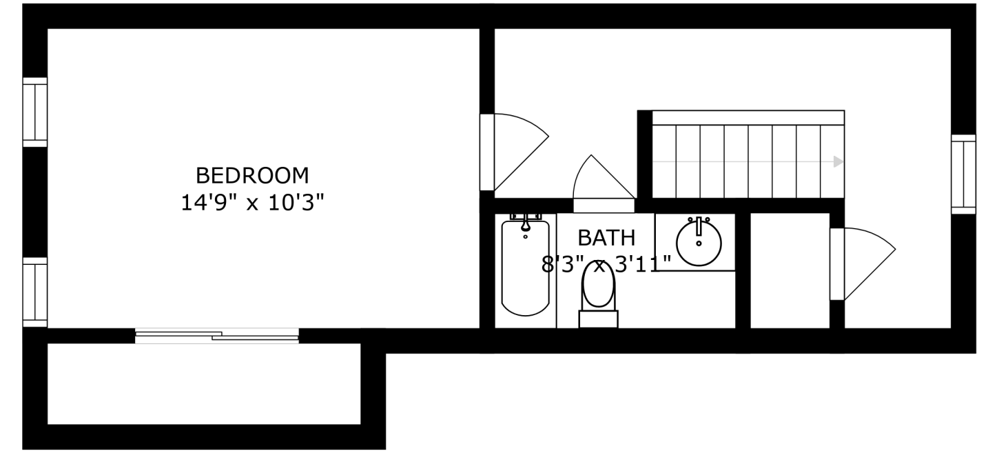
FLOOR 4
