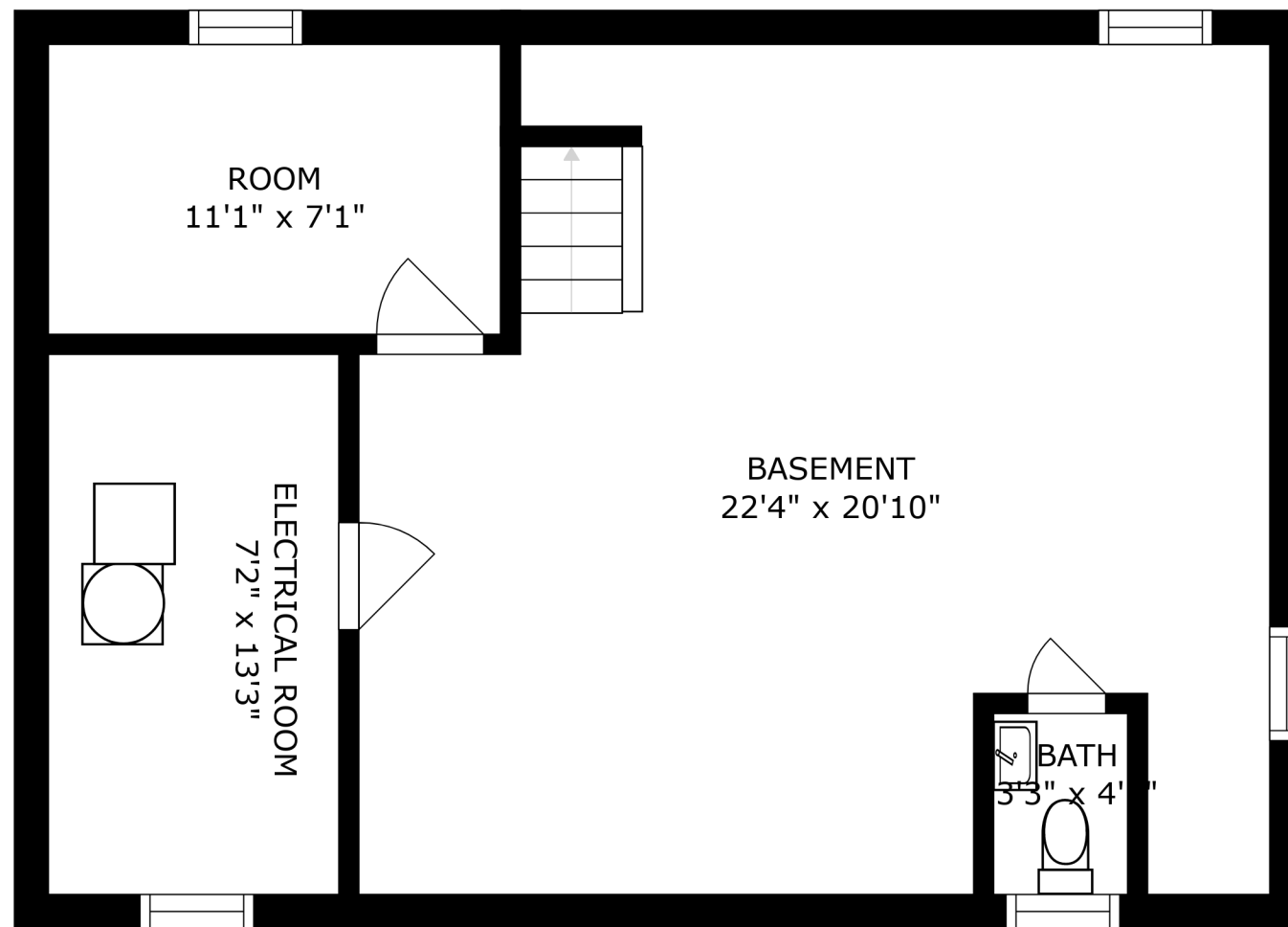
FLOOR 1
