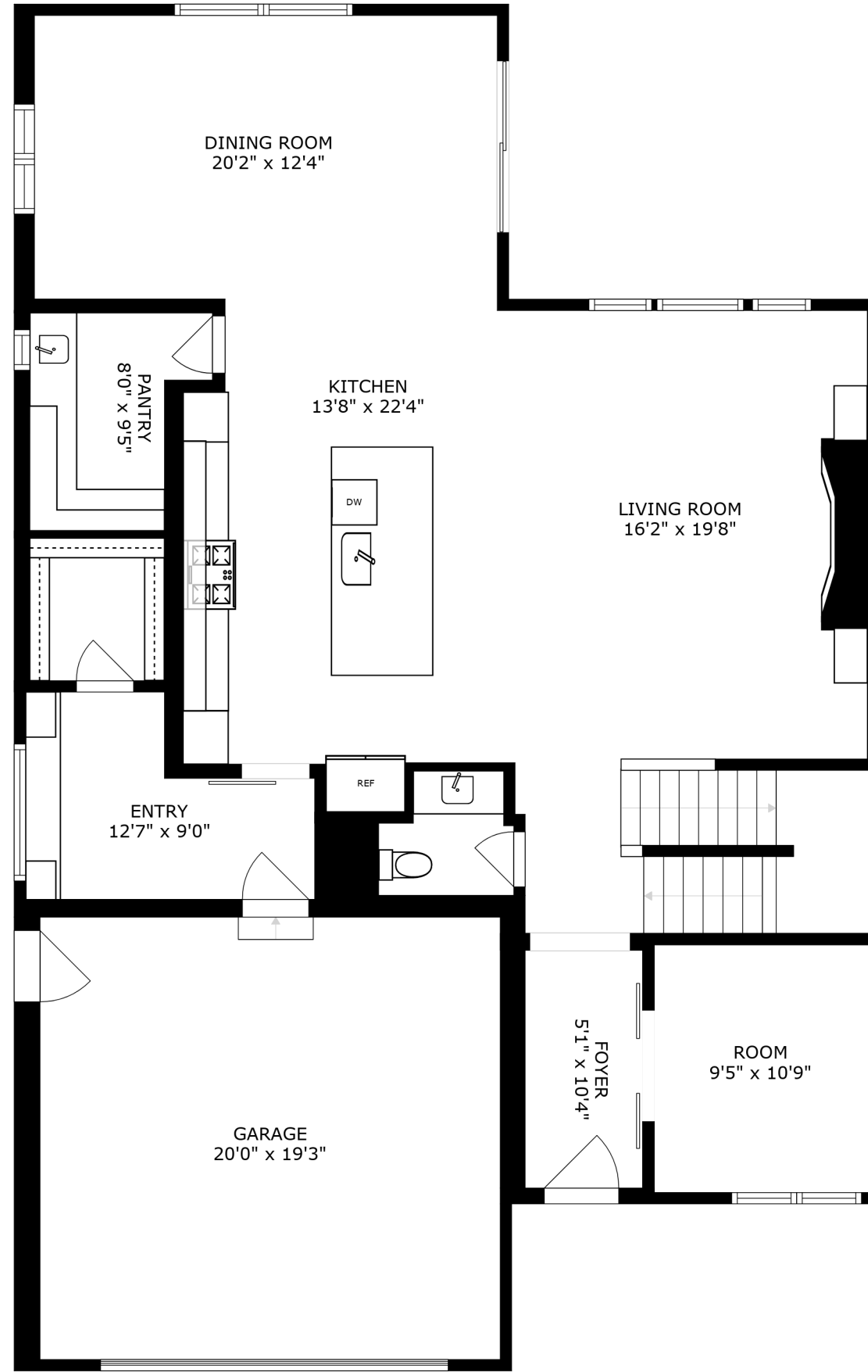
FLOOR 2
