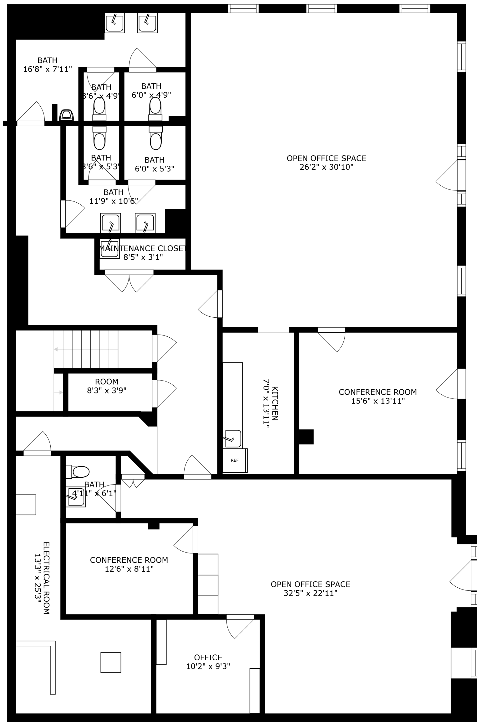
FLOOR 1
