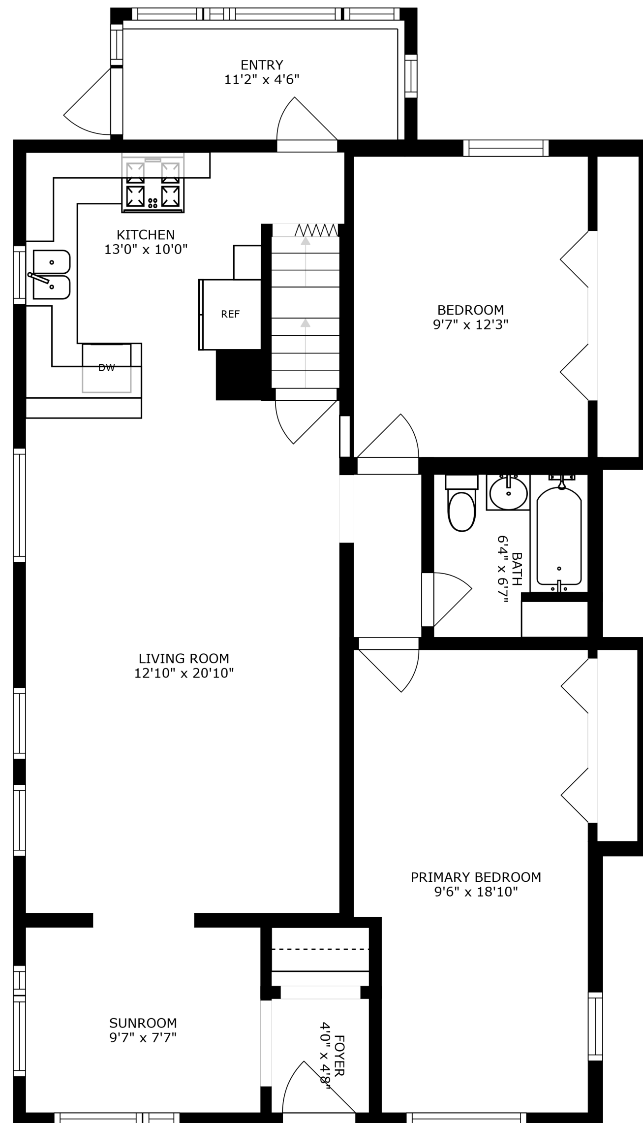
FLOOR 2
