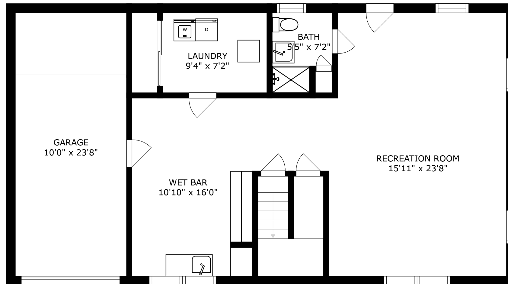
FLOOR 1
