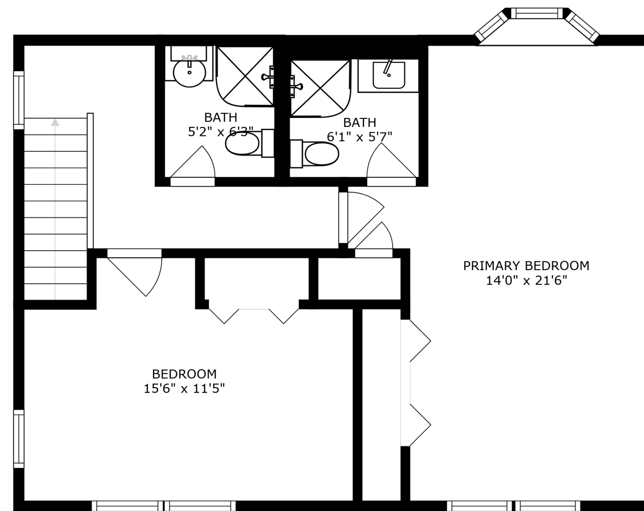
FLOOR 3
