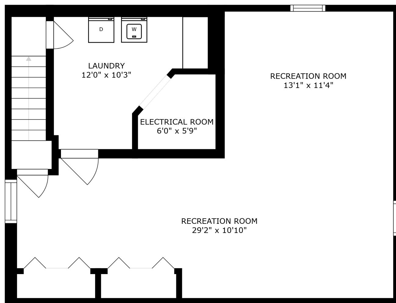
FLOOR 1
