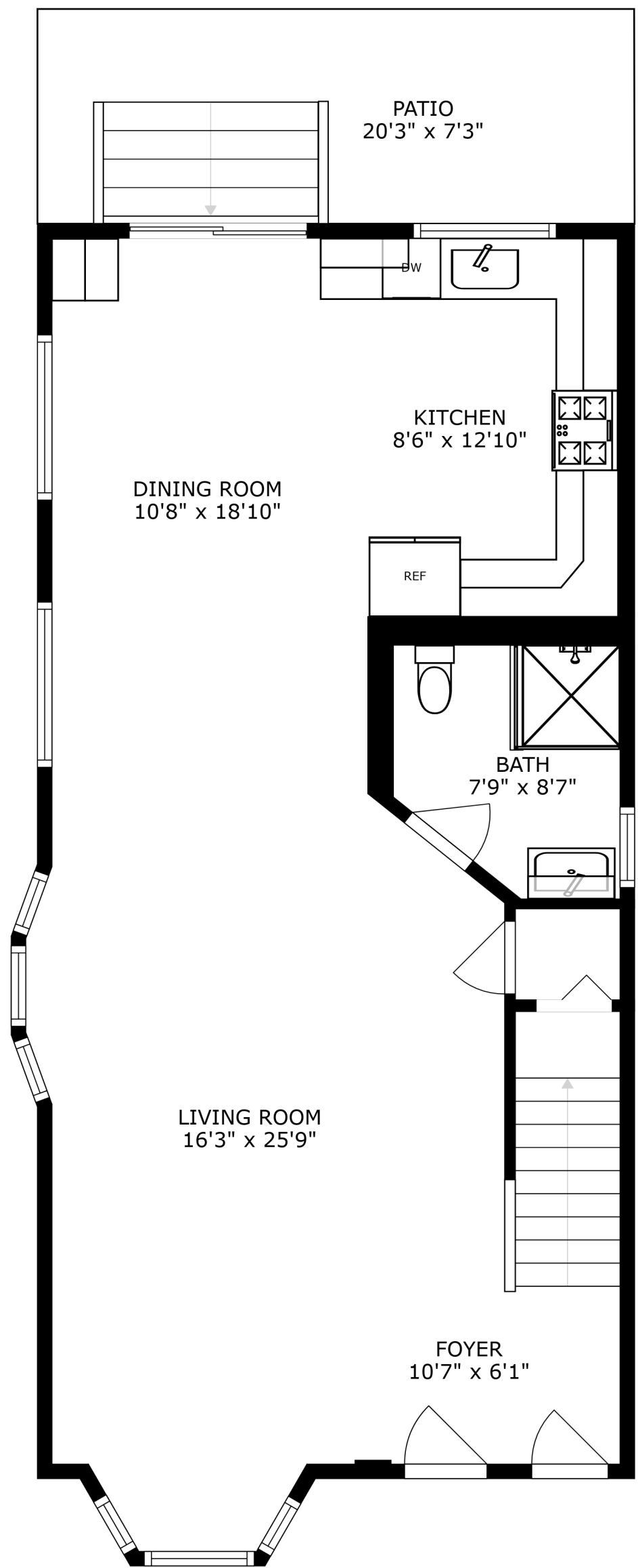
FLOOR 1
