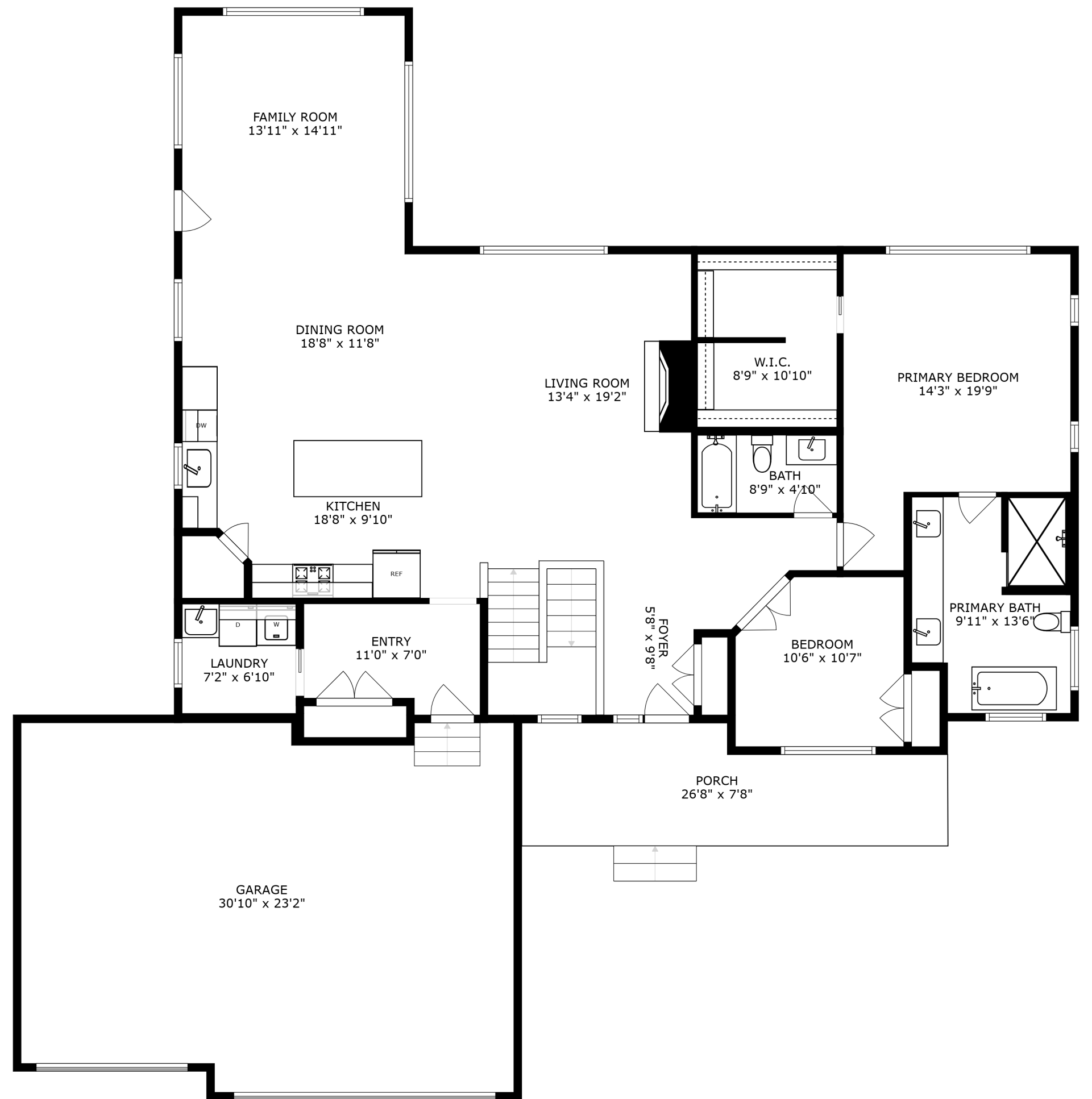
FLOOR 2
