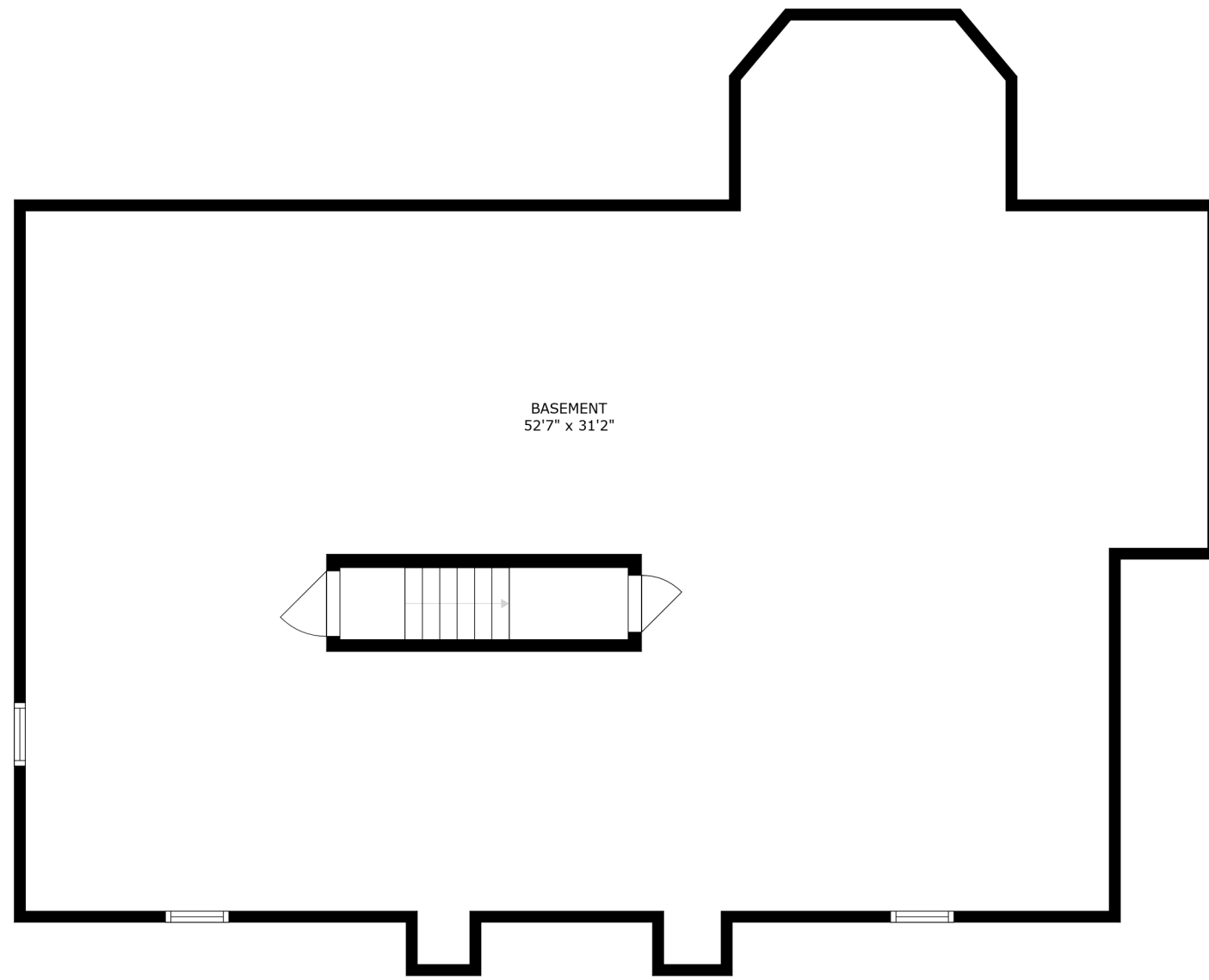
FLOOR 1
