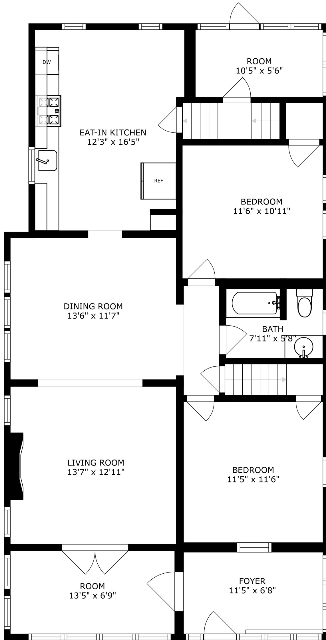
FLOOR 2
