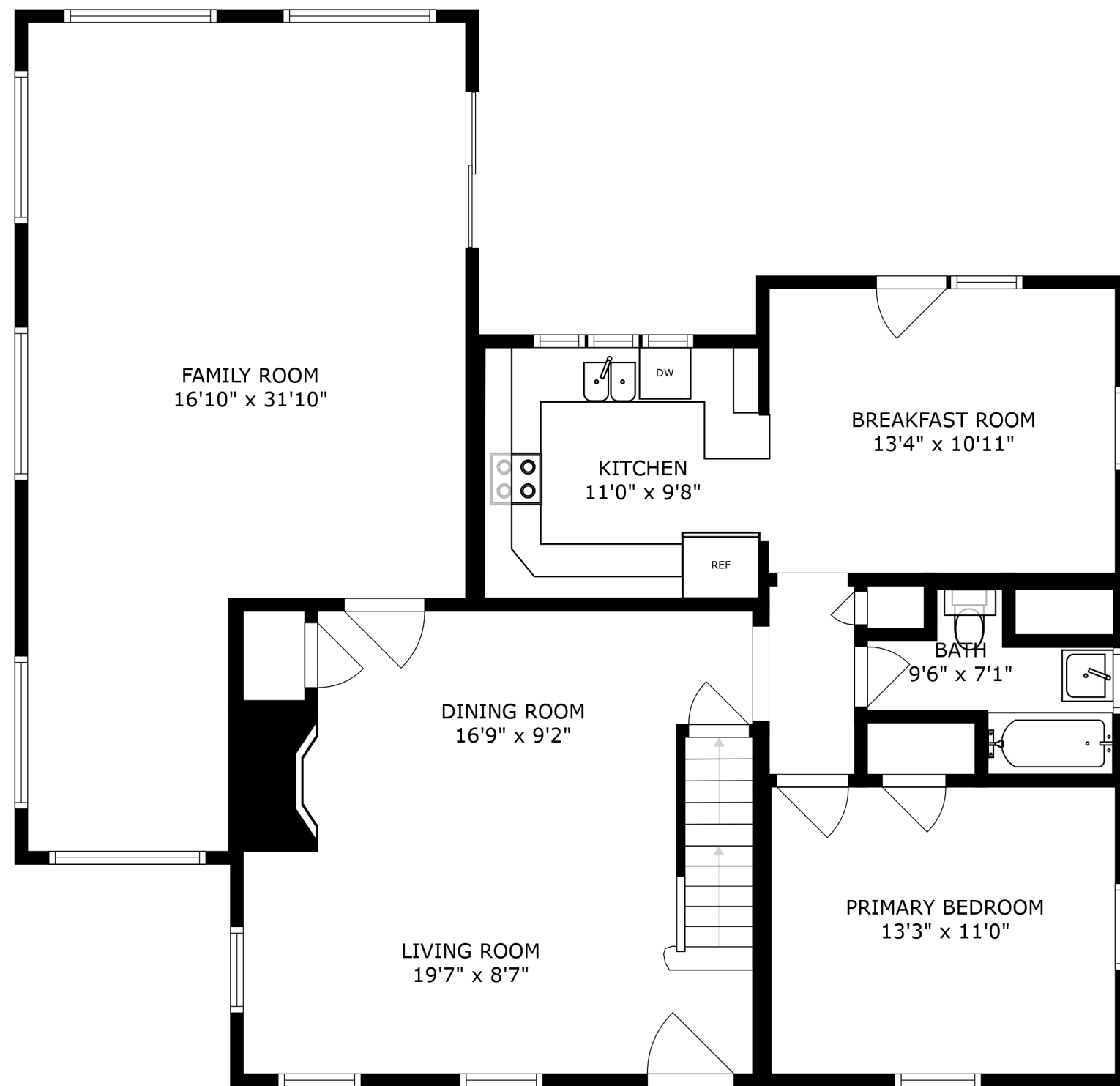
FLOOR 2
