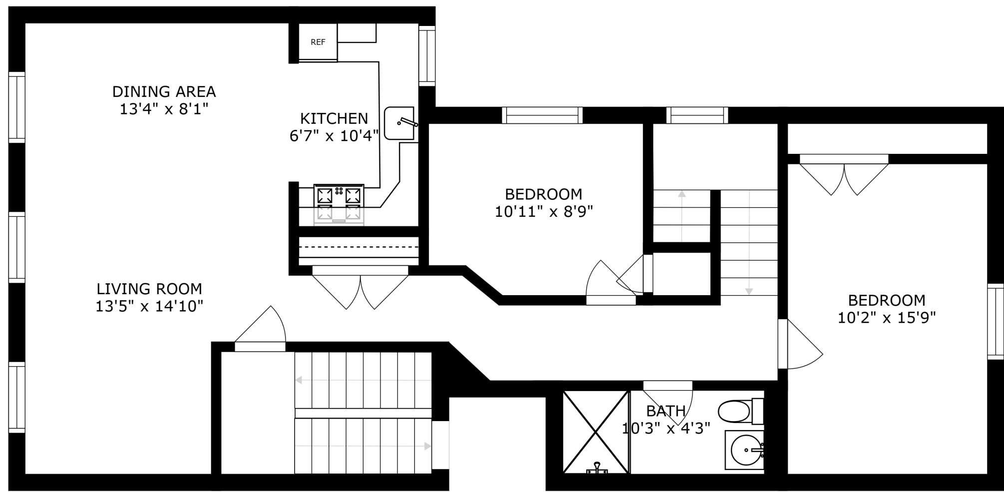
FLOOR 3
