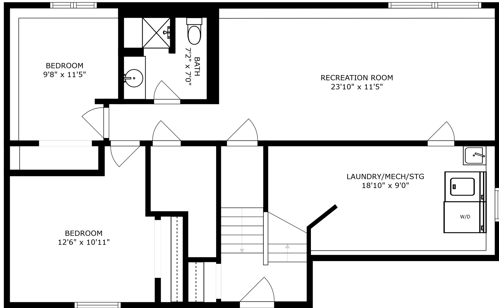
FLOOR 1
