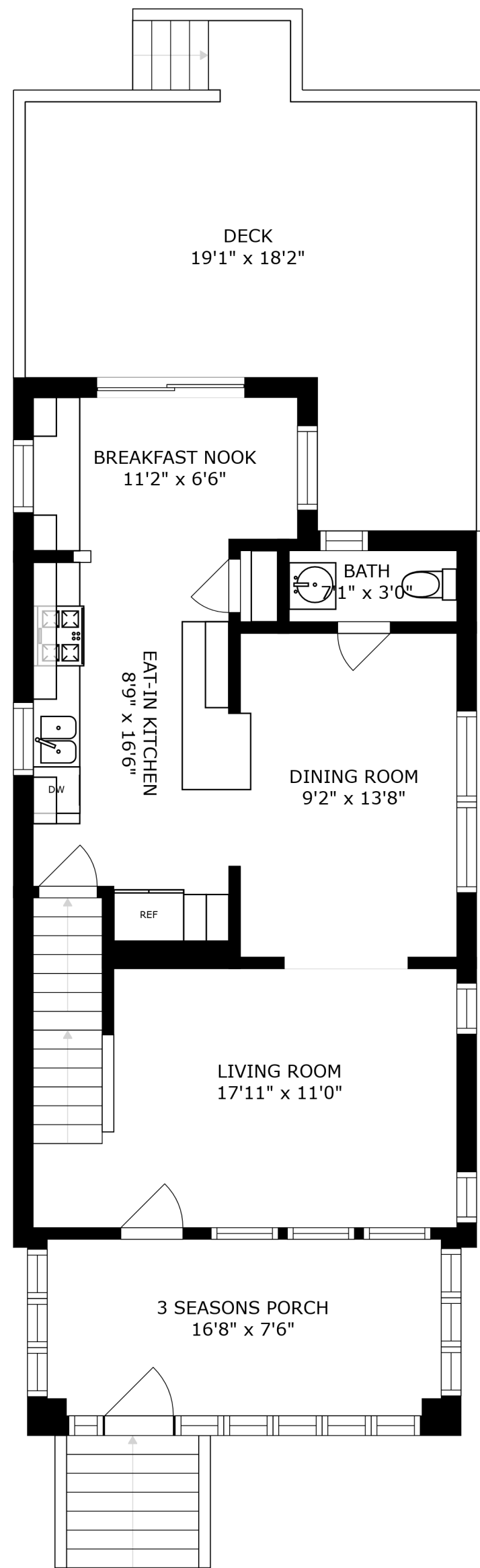
FLOOR 2
