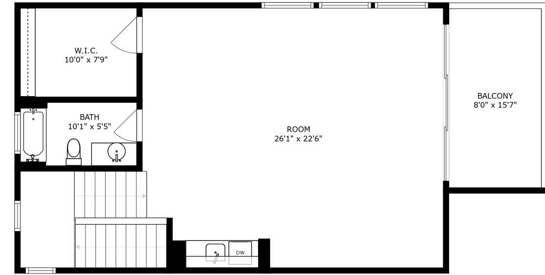
FLOOR 2
