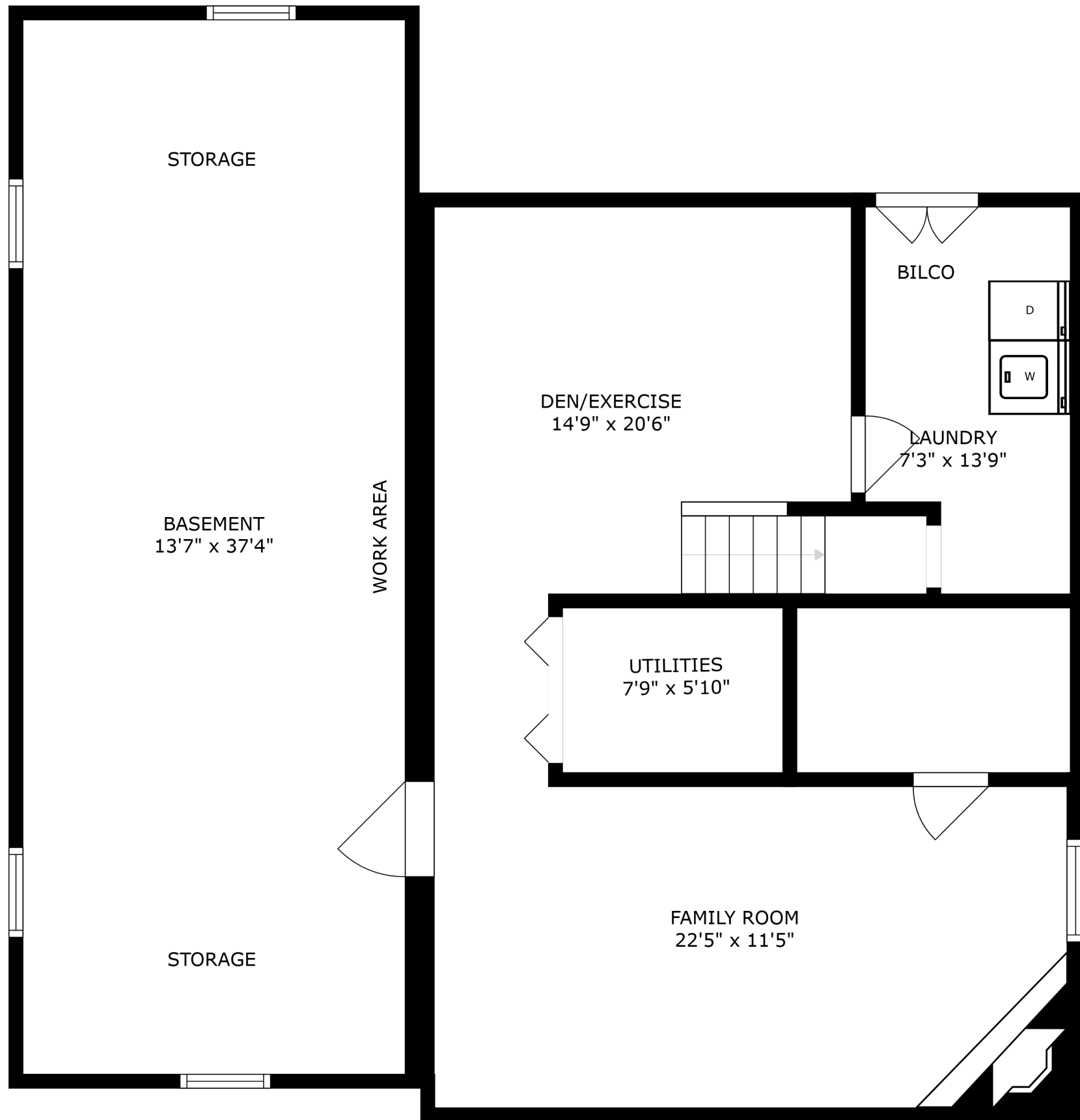
FLOOR 1
