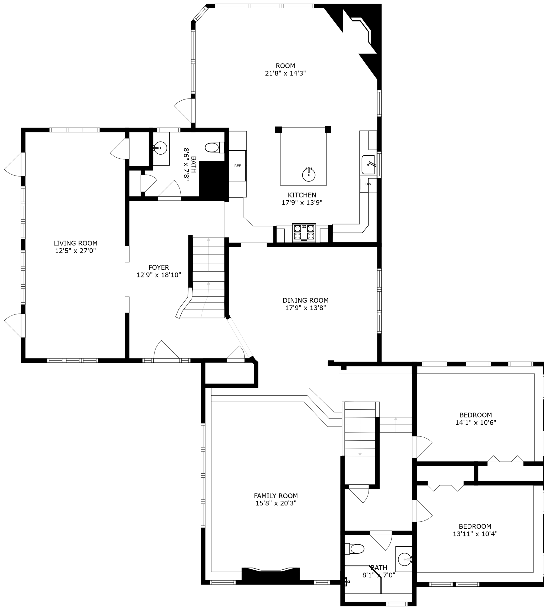
FLOOR 1
