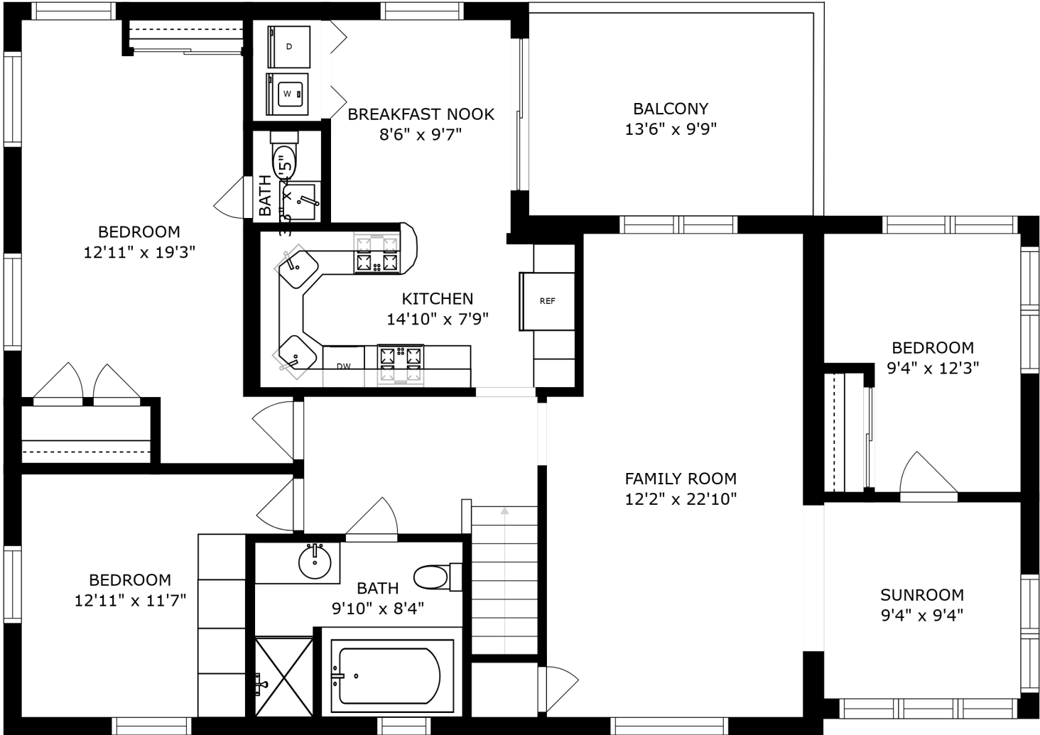
FLOOR 3
