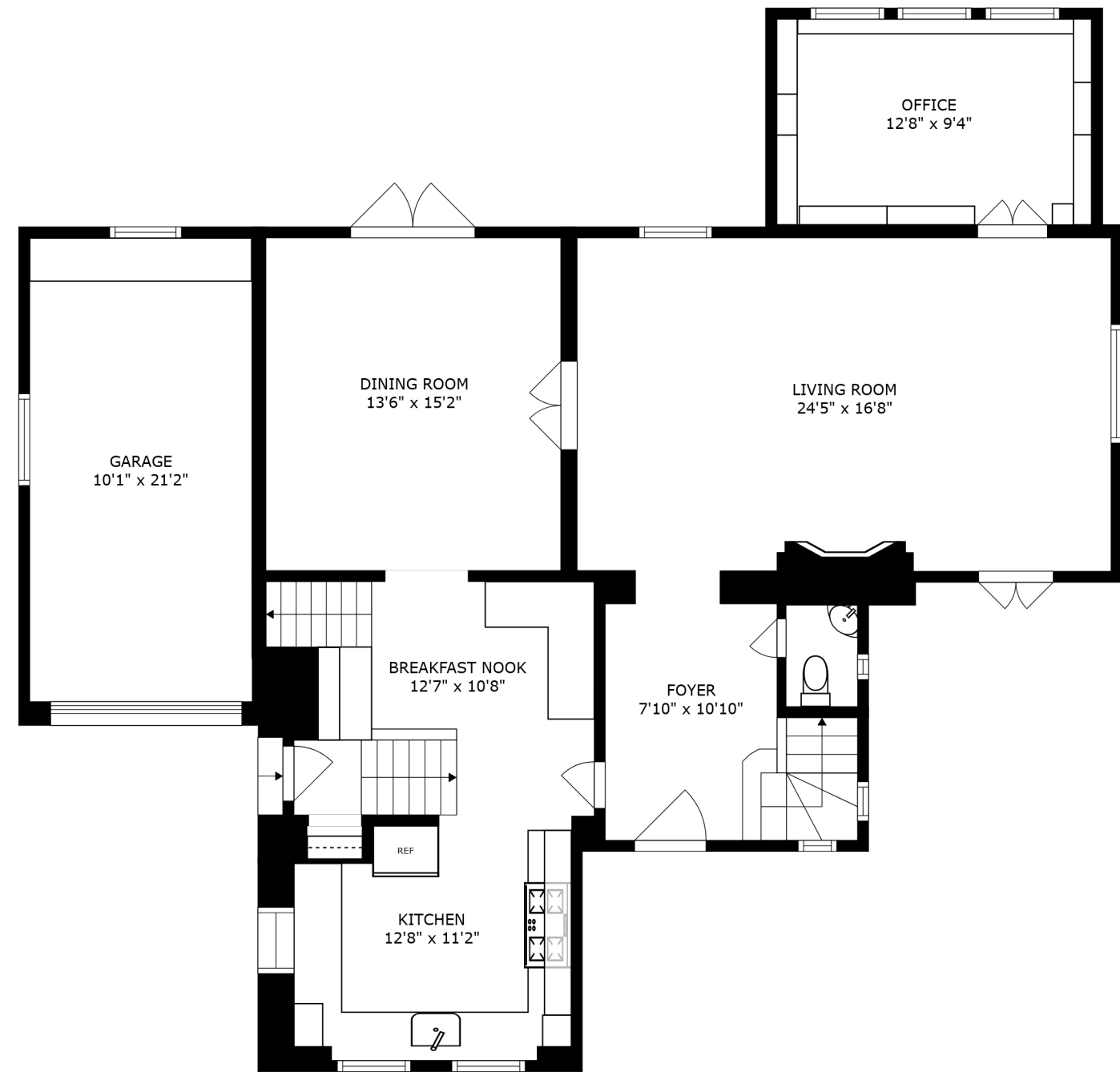
FLOOR 2
