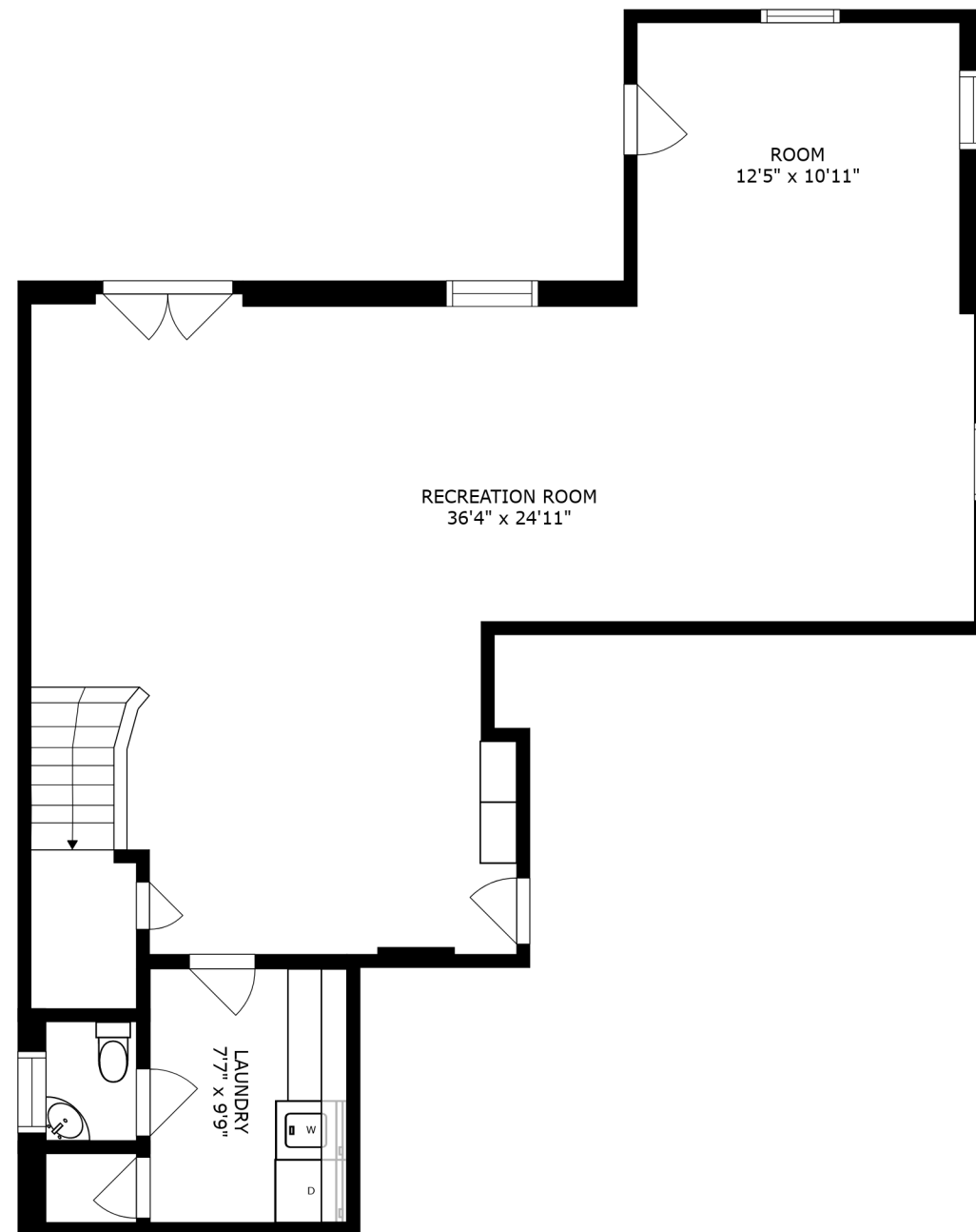
FLOOR 1
