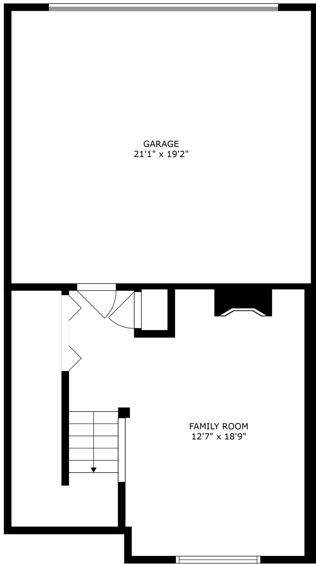
FLOOR 1
