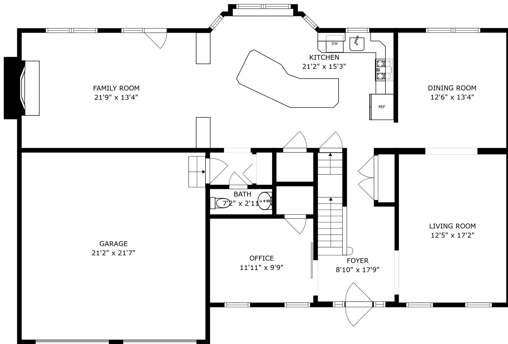
FLOOR 2
