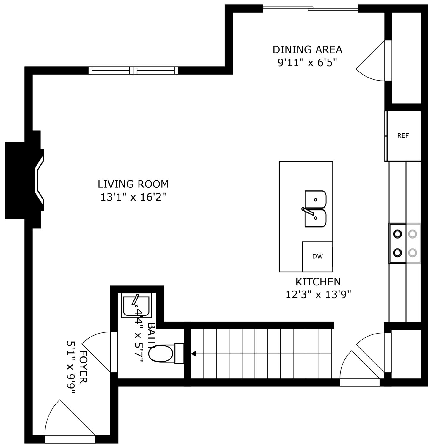
FLOOR 1
