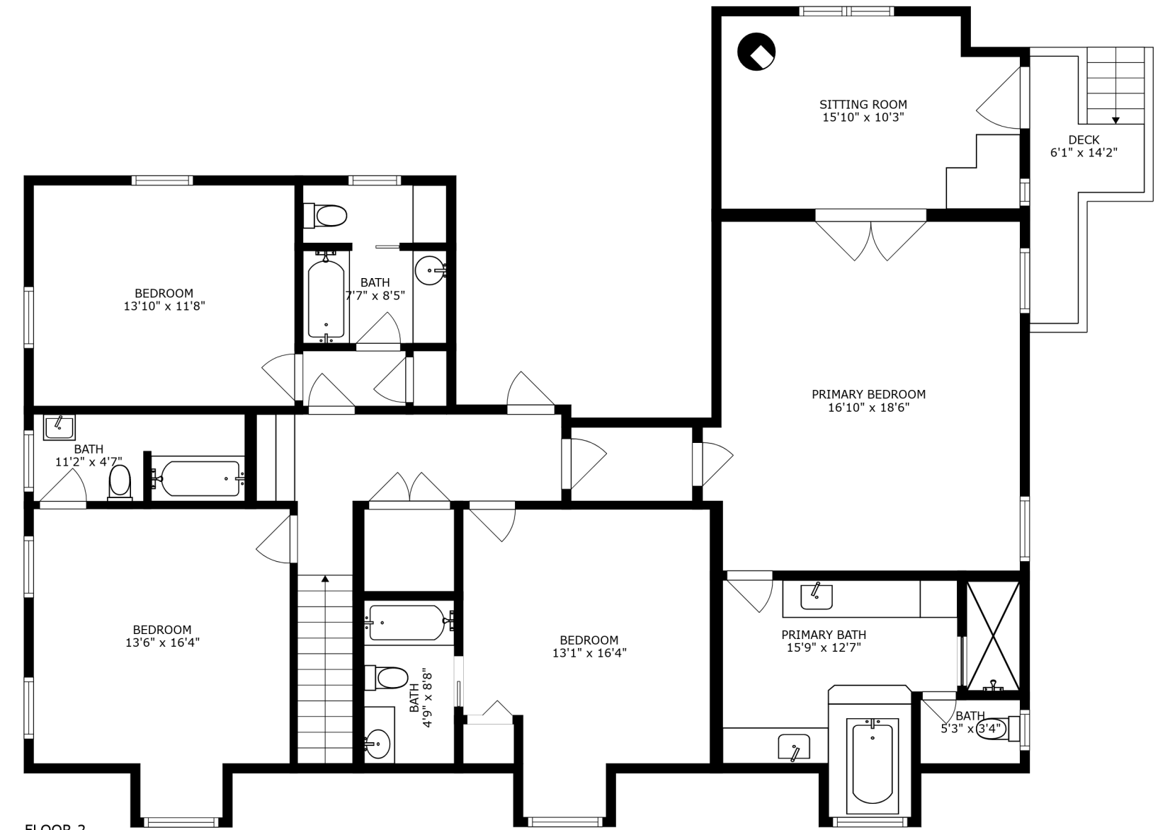
FLOOR 2
