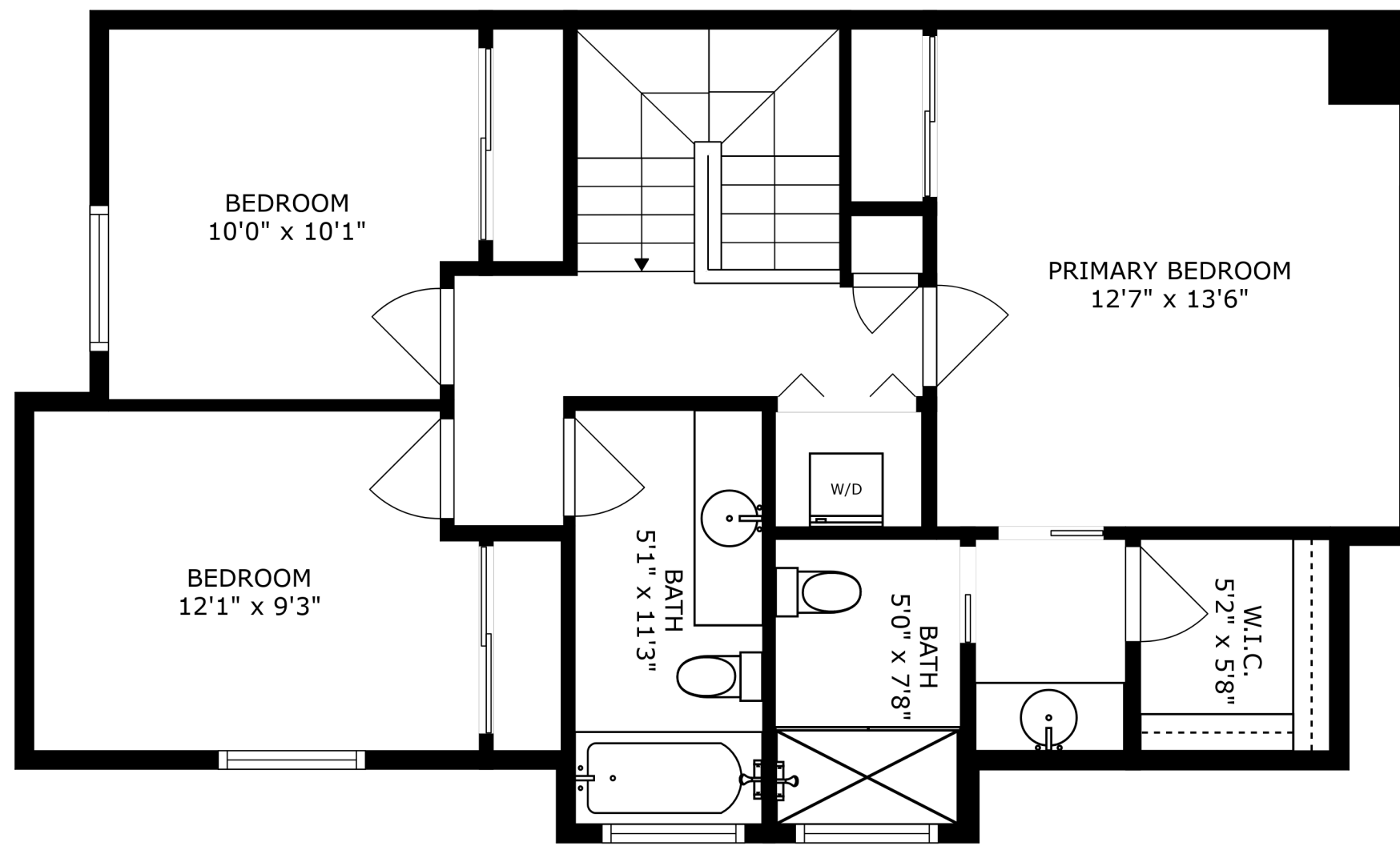
FLOOR 2
