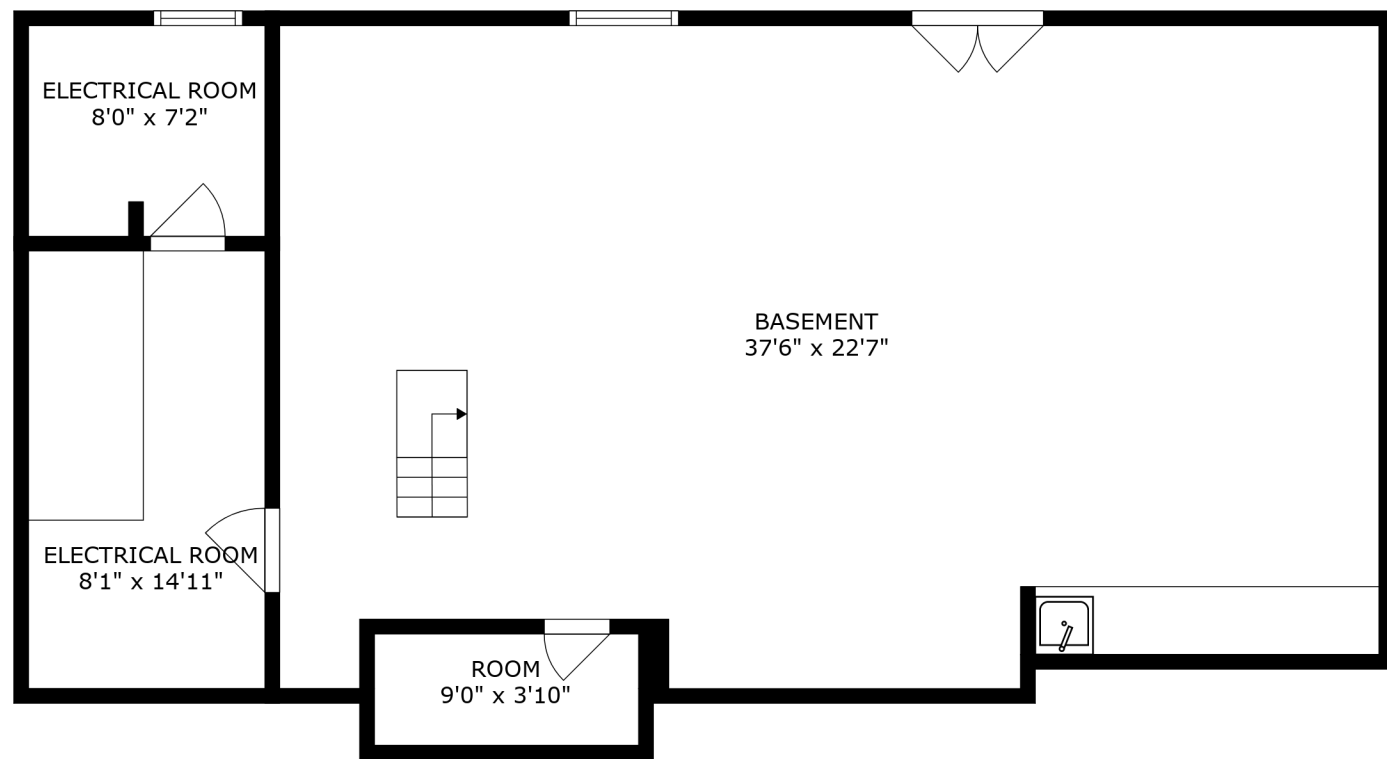
FLOOR 1
